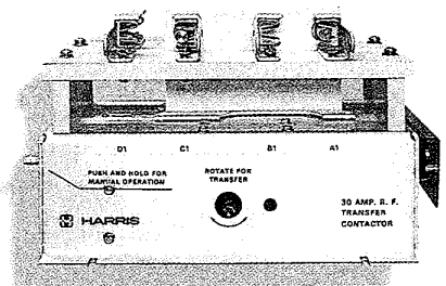
HS-4P 30 Amp RF Contactor
