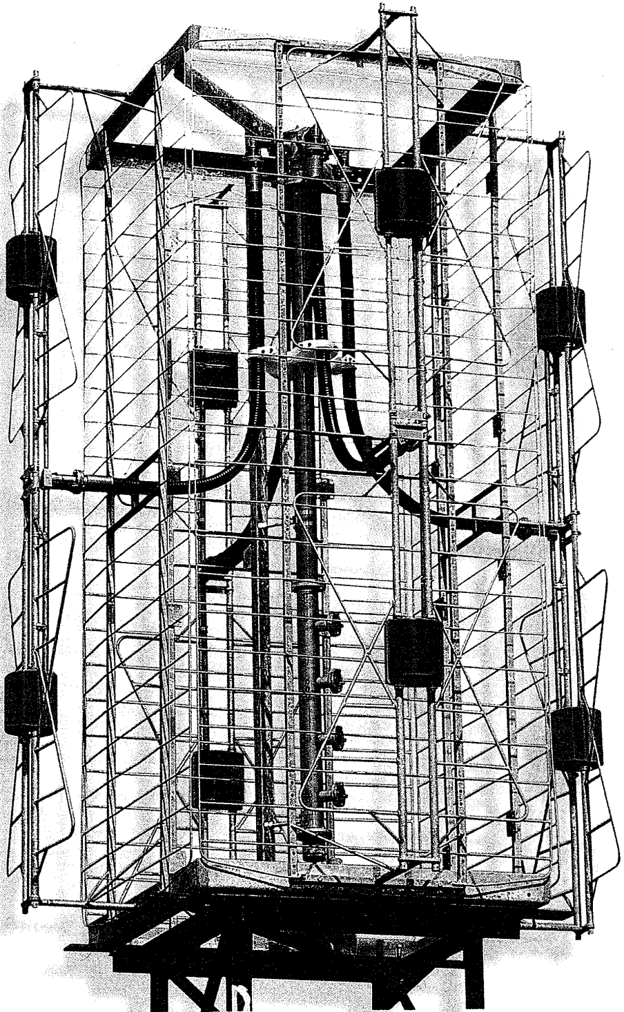
Harris VHF TAD-HDAHP Duplet Deltawing Array
