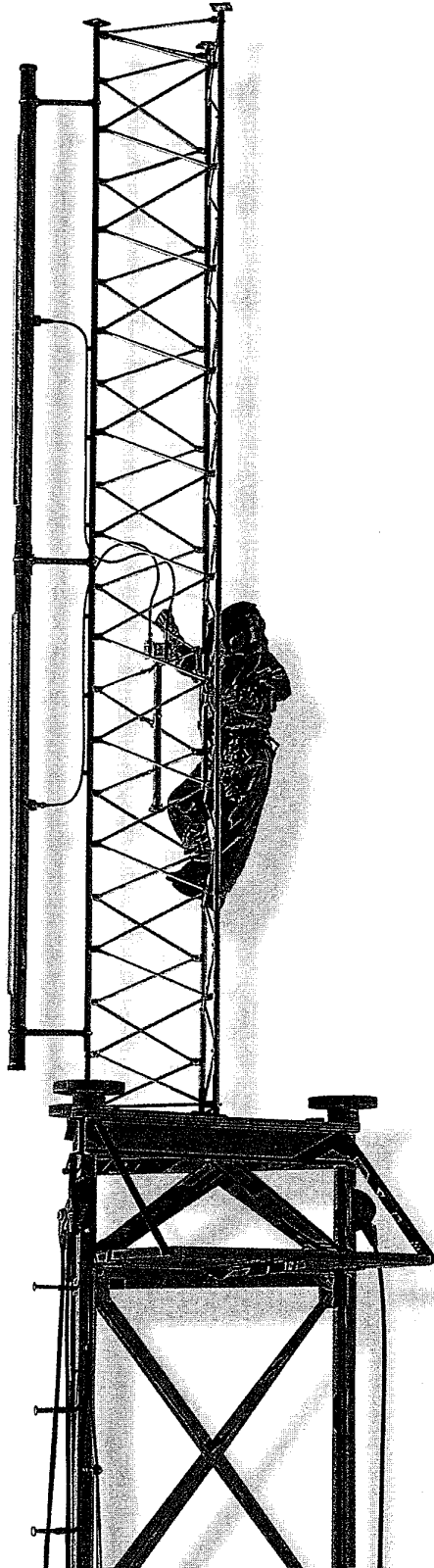
Harris Medium Power TWS-LP Side-Mount UHF Antenna
