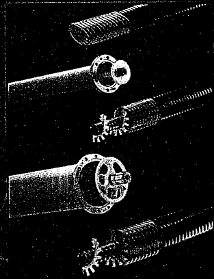
HELIAX® Coaxial Cable and Waveguide
