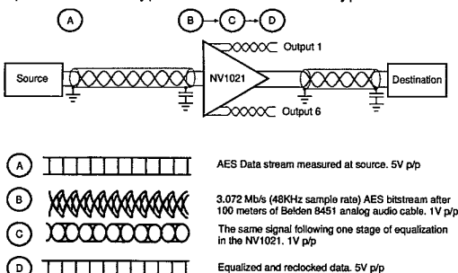
Figure 3. Cable Equalization
