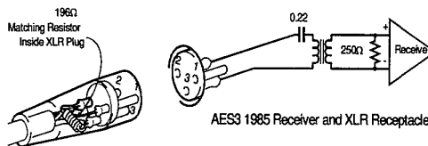
Figure 1: Impedance Correction of AES3 1985 Receivers
