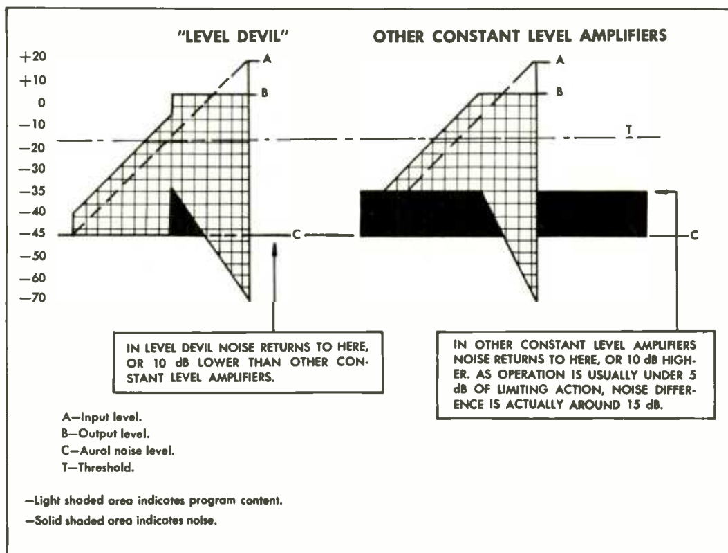
A graphic illustration of the difference between Level Devil and all other leveling amplifiers. Noise referred to in graphs is defined in this instance as lower level program content.
