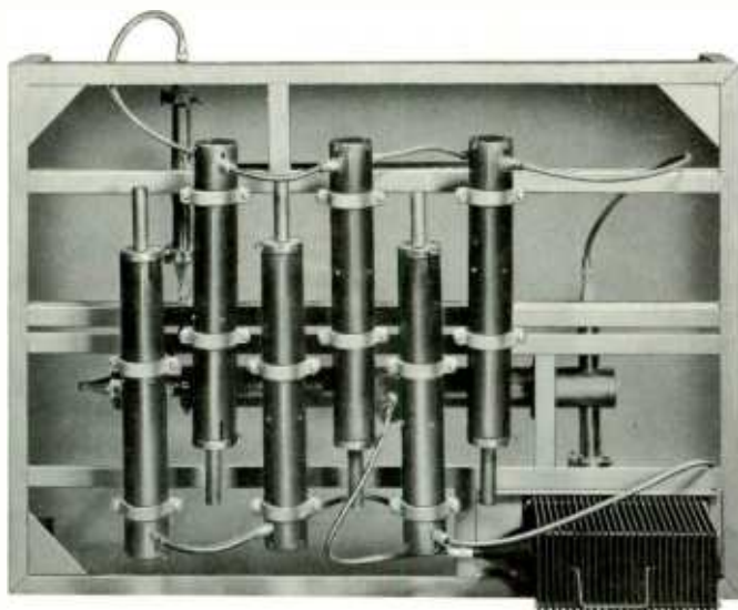
The vestigial sideband filter above, employed at the output of the visual amplifier, is supplied with the BT-500C VHF transmitter as standard equipment.
