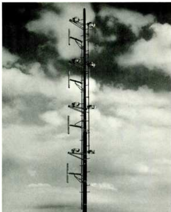
Directional FM antenna as supplied by Gates to Radio Station WMSH, Hershey, Pennsylvania. Antenna consists of four bays directional Cycloid and four bays non-directional 300G elements.
