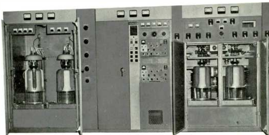
Three main transmitter cubicles house (from left to right) the modulator, transmitter control circuitry, and RF power amplifier.
