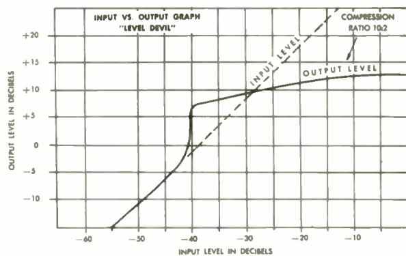
Graph shows compression or limiting curve as related to input.
