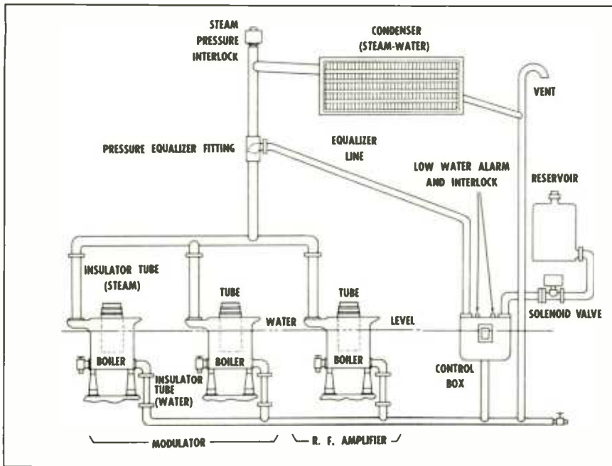
Vapor Phase Cooling.
