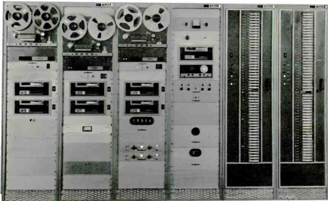
This system, designed for a large major market broadcaster (FM) in New England, handles varied programming through a combination of reel-to-reel tape machines, Criterion cartridge decks and Criterion 55 multiple cartridge reproducers. The system also employs automatic program logging (not shown).
