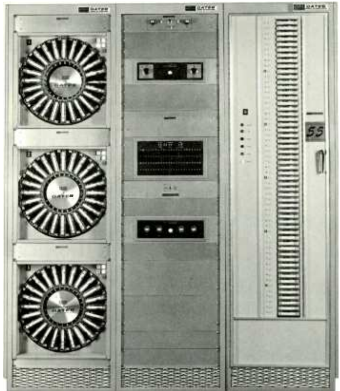
Small but highly flexible Gates automation system now being used successfully by a 3 kW Gulf Coast FM station. The system handles a "Top 40" format, and features automatic network joining with ABC for news and features.
