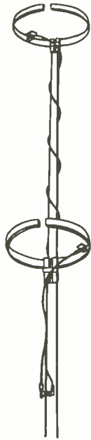
Left, FM-11 single ring omni-directional antenna with power gain of 0.8 dB. Right, two bay FM-22 omni-directional antenna with gain of 1.6 dB. These are broadband, easy to install antennas.
