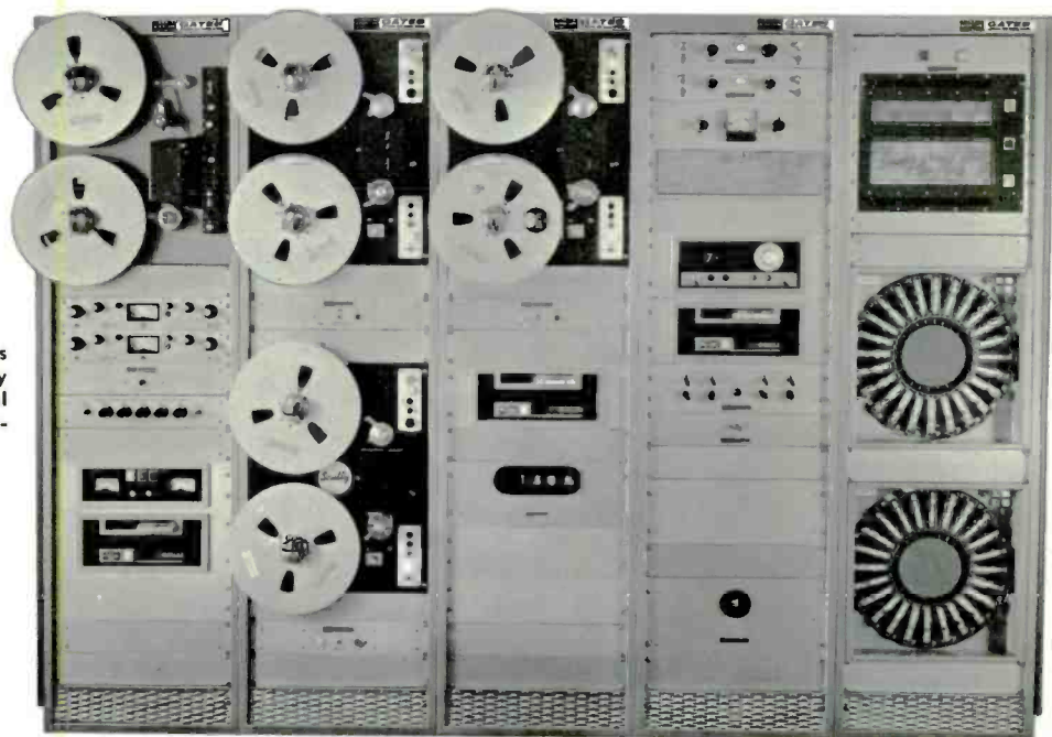
A new AM station in the west has employed this semi-custom automation system since its first day on the air. Note the extensive use of reel-to-reel tape machines—planned by Gates to fit the station's middle-of-the-road format.
