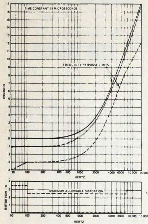
Stereo: Right Channel Response and THD
