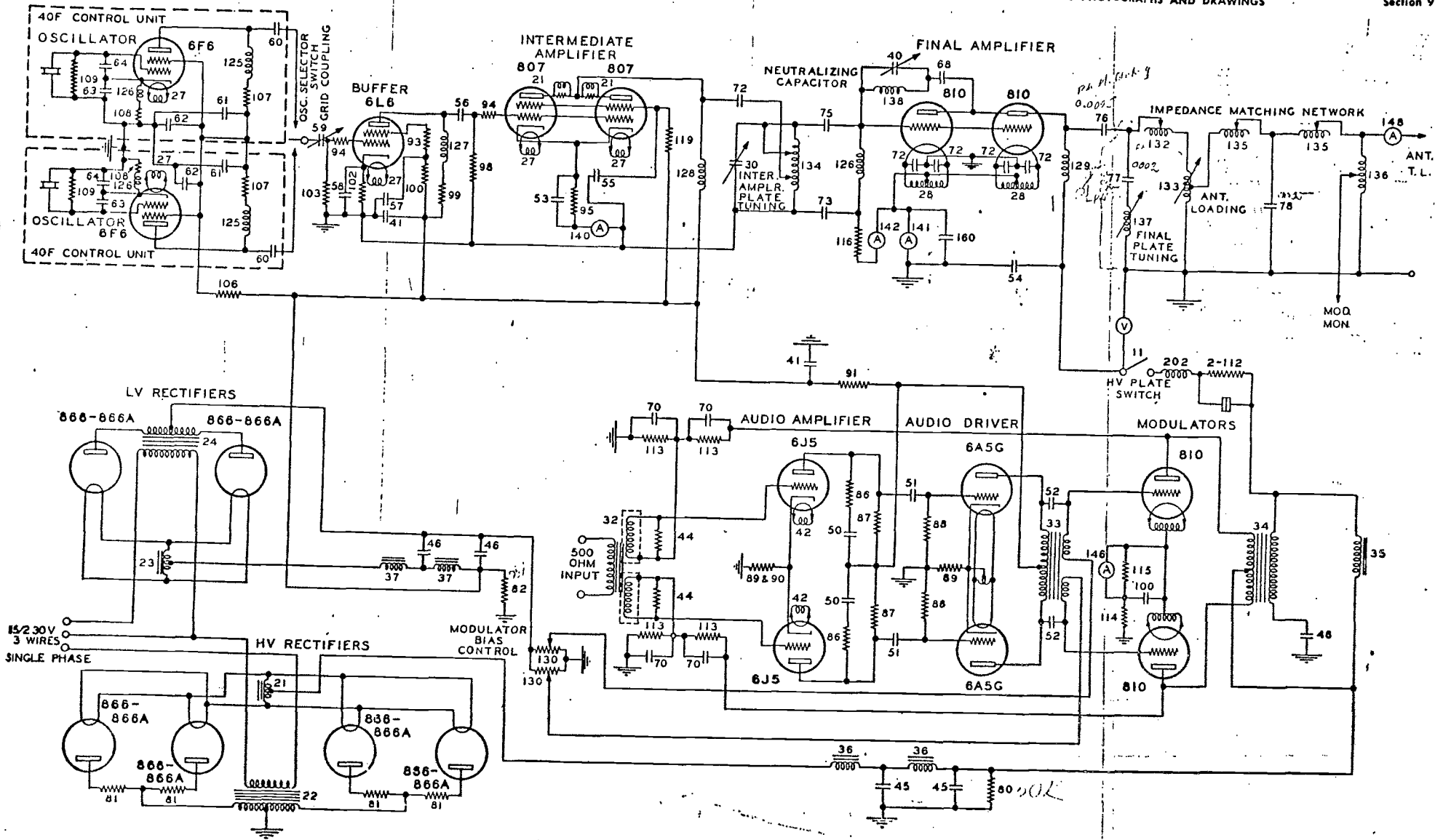
Figure 9-8. 300G Simplified Schematic
