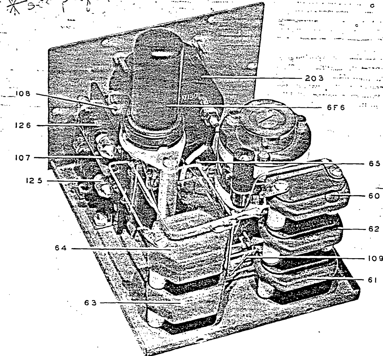
Figure 2-10. 40F Frequency Control Unit - Open View
