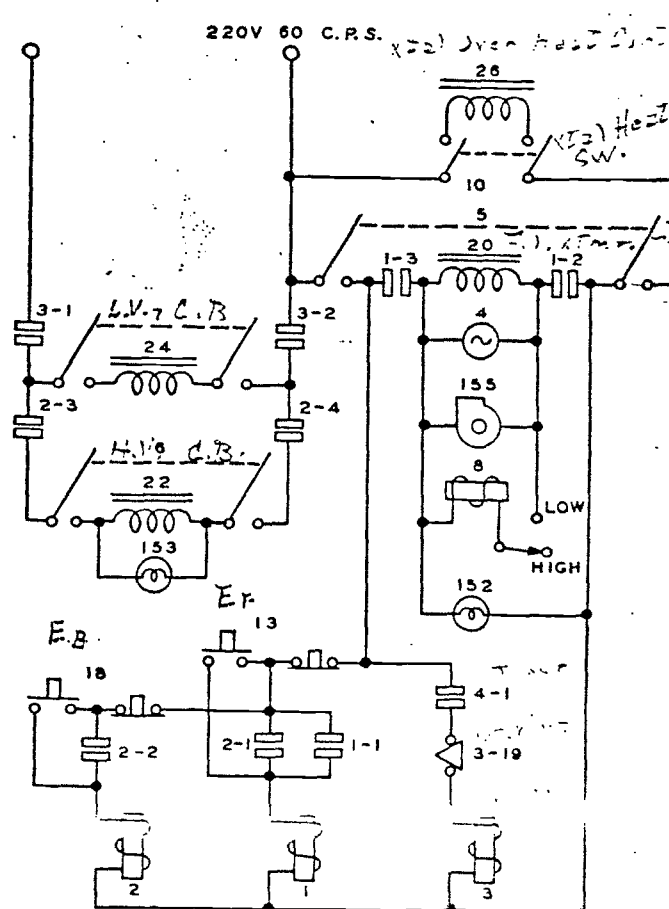
Figure 2.5. Power Control Circuits
