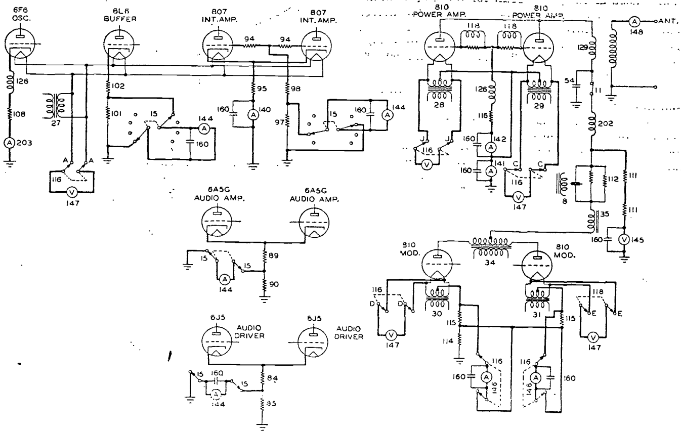
Figure 2-13. Metering Circuits
