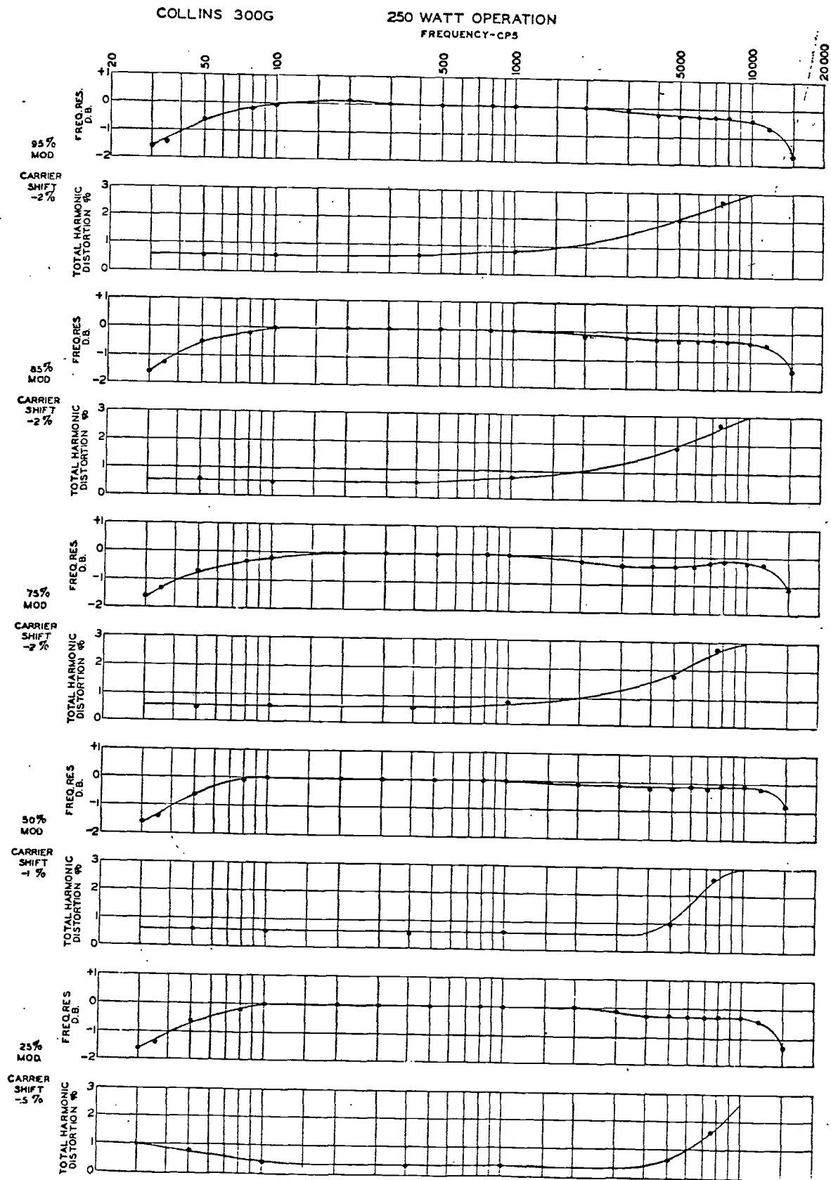
Figure 8-2. Audio Frequency Response and Distortion Curves for 250 Watt Operation
