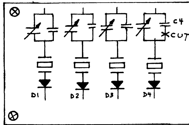
FIX-VOX BOARD
