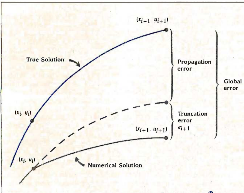
Figure 1: An illustration of errors in a numerical solution.
