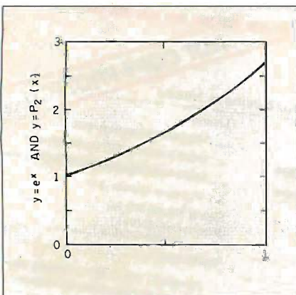
Figure 2: A graph of \exp(x) for x=0 to 1. Included is the best-fitting polynomial of degree 2.
