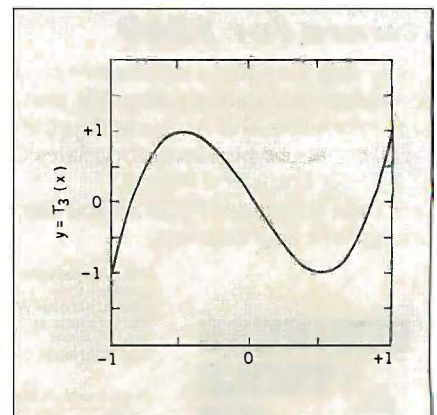
Figure 4: A graph of the Chebyshev polynomial of degree 3.
