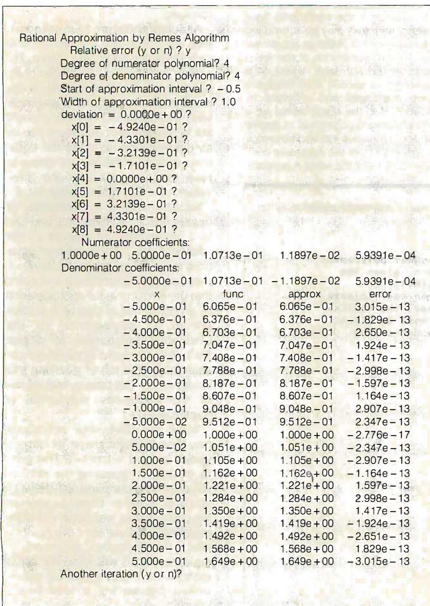
Figure 5: An interactive session with the author's Remes program. The approximation is for the exponential function.
