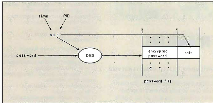
Figure 3: UNIX password encryption. When the user enters a new password, it is encoded by a variant of the DES algorithm. The algorithm is modified in one of 4096 different ways by a random quantity called the salt, which is then stored in the file /etc/passwd along with the encrypted password.
