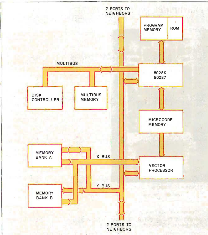
Figure 2: The architecture of a single node of our machine. Only the major elements of the design are shown.
