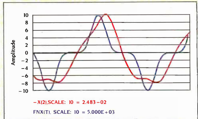
Figure B: A graph of displacement (X(2)) and driving force (FNx(T)) versus time for the startup of the system with Coulomb damping.
