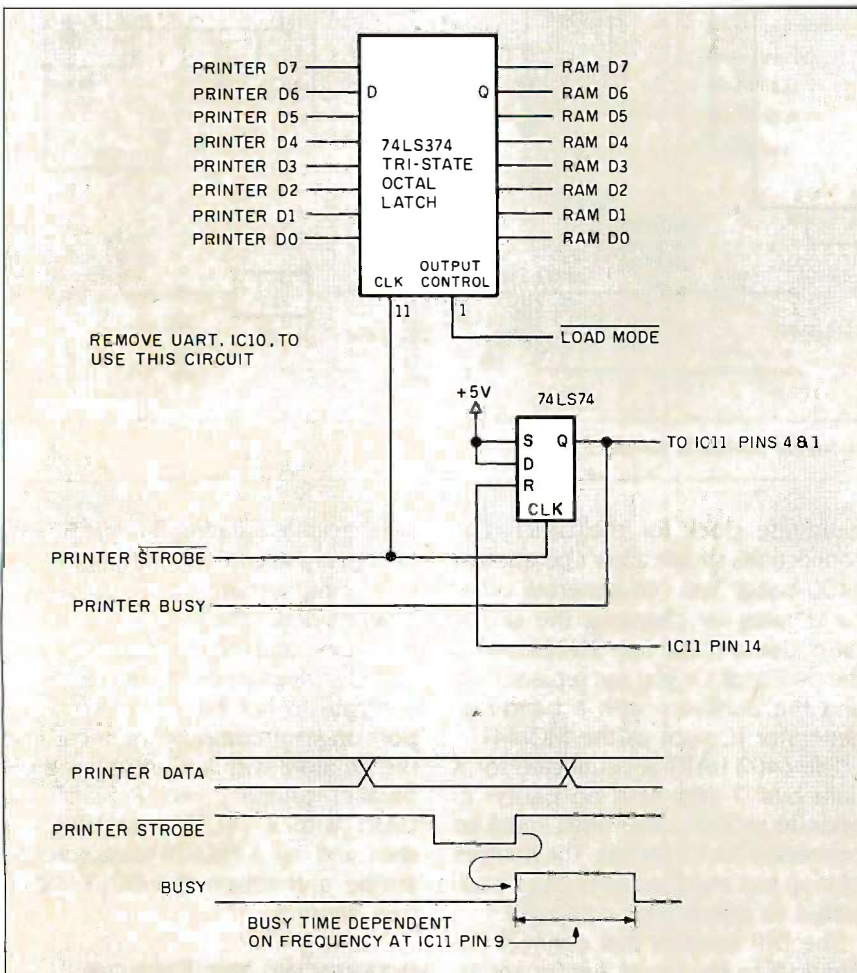
Figure 3: Schematic for interfacing the Emulo-8 to a printer port with the load timing using the printer interface.
