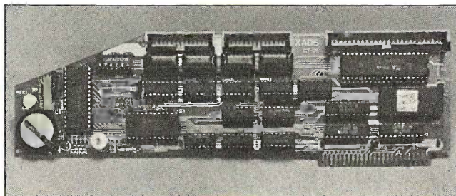
Xcalibur's XAD5 data-acquisition board.
