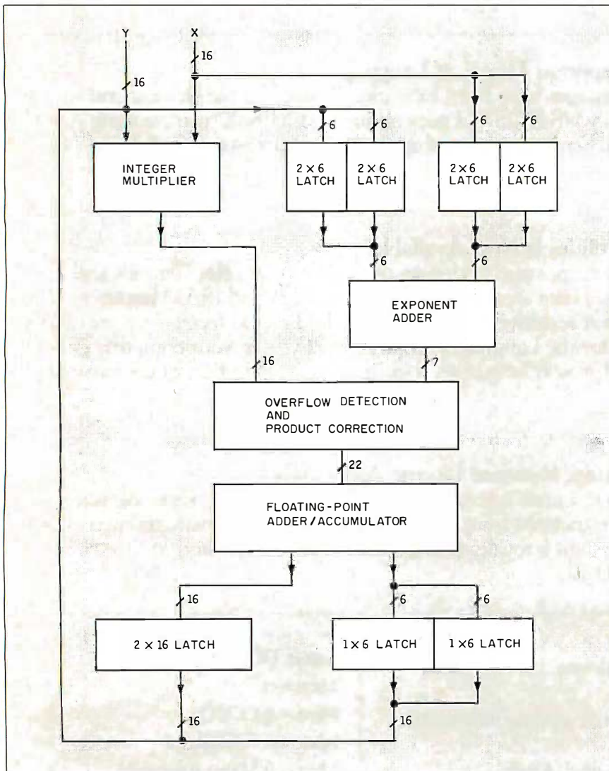
Figure 5: The configuration of adder, multiplier, and latches making up a vector processor.
