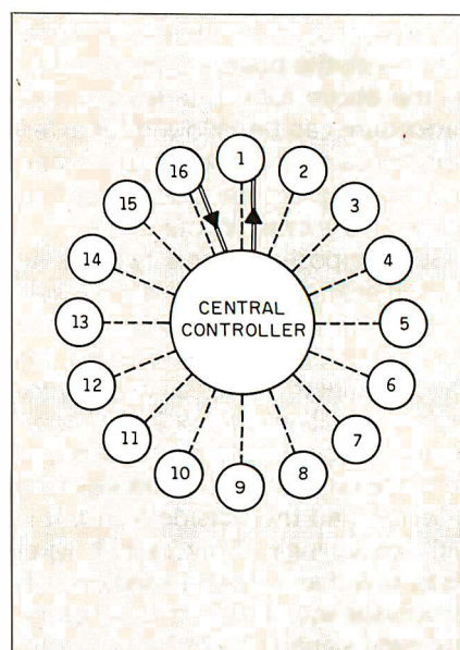
Figure 4: The radial connection between the central controller and the parallel nodes. The doubled lines refer to the data paths between the controller and the first and last nodes of the I/O bucket brigade.
