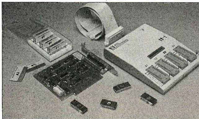
Avel Electronics' EP-4 PROM gang programmer.
