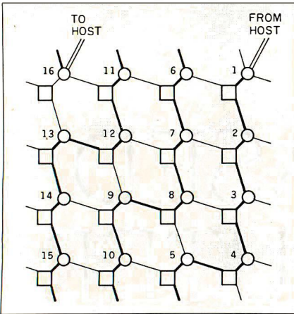
Figure 1: The interconnection scheme for 16 nodes. The squares represent data memories, and the circles represent processors.
