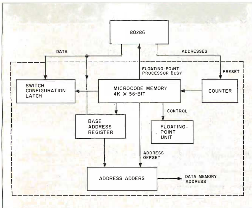
Figure 6: The arrangement of the control system for the floating-point unit. That portion inside the dashed box makes up the elementary microcode control that can operate concurrently with the 80286.
