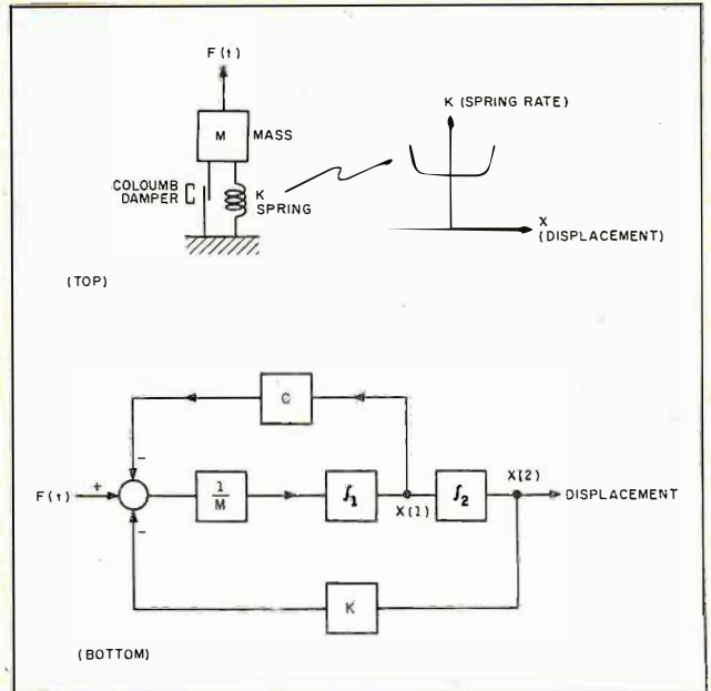
Figure A: The top of this figure shows a mechanical model of a damped spring-mass system. The bottom shows a block diagram of an analog model equivalent to the mechanical model.
