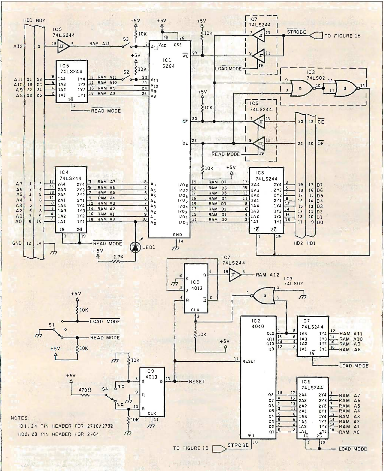
Figure 1a: A schematic diagram of the Emulo-8.
