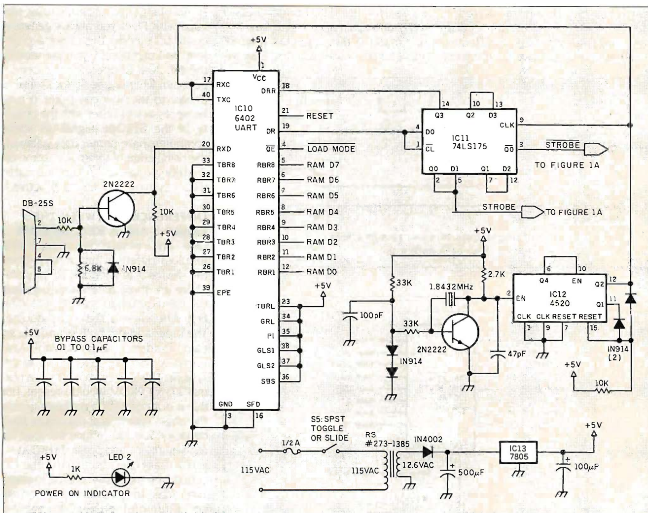
Figure 1b: Serial interface circuitry and power supply schematic for the Emulo-8.
