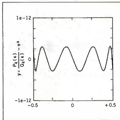
Figure 6: The error curve for the approximation solved in figure 4.
