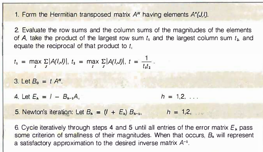
Figure 2: An outline of the Pan and Reif method discussed in the article.
