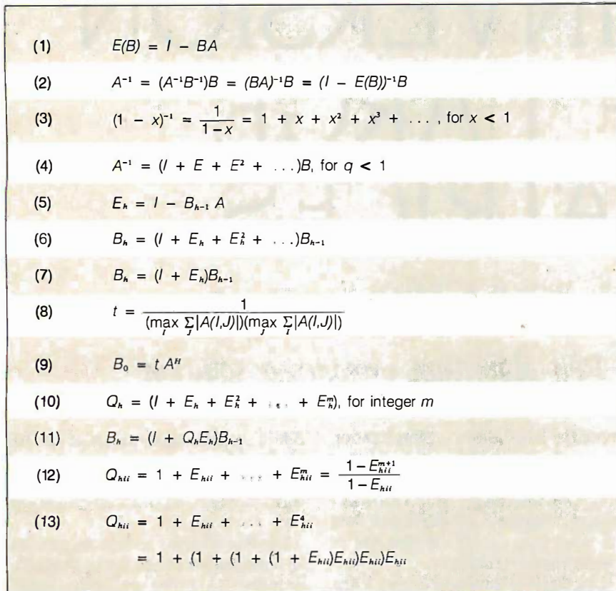
Figure 1: Equations used in the article.
