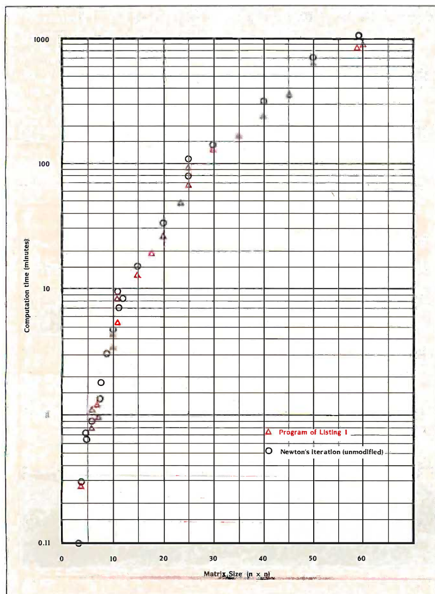
Figure 3: A plot of log (computation time) versus matrix size.
