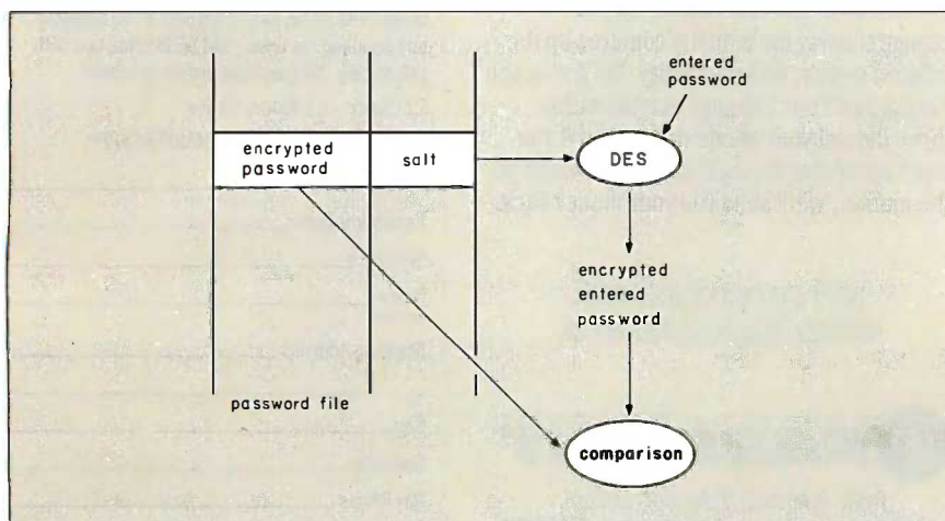
Figure 4: UNIX password verification. The entered password is encrypted by a variant of the DES algorithm using the salt string readout of the /etc/passwd file entry for that user. The resulting encrypted password is compared to the encrypted password in the file. If they are the same, the password is accepted. Note that the password in the file is never "decrypted."
