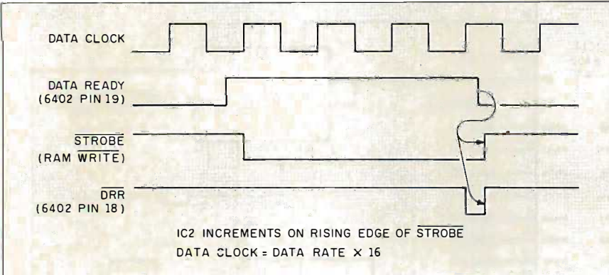
Figure 2: RAM load timing.
