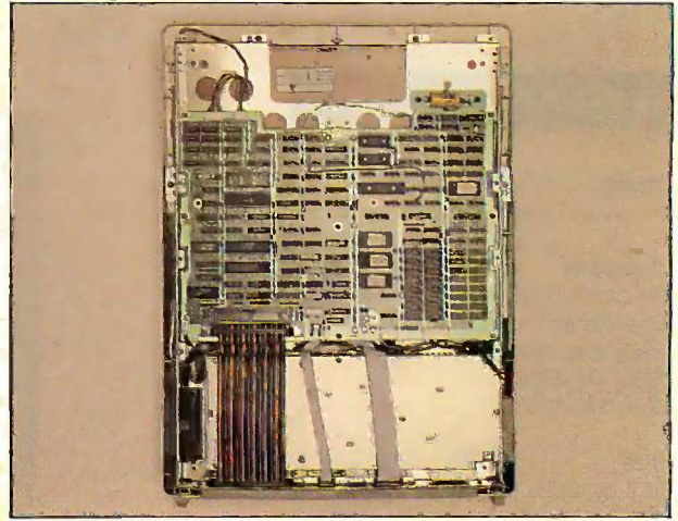
Clockwise from bottom to top: the Exec. Partner's power supply with cooling fan, ribbon cable to expansion connector, and the motherboard.
