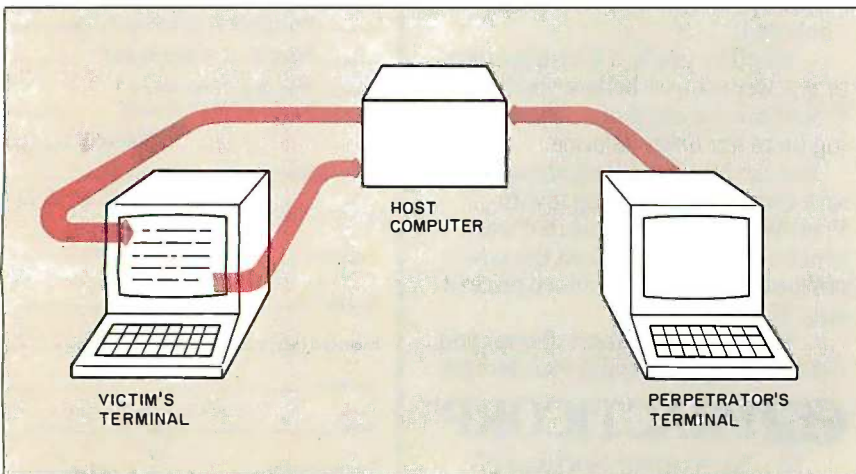
Figure 5: Terminal page-mode buffering. The colored path indicates how the perpetrator can send his or her own commands to the victim's terminal and then to the host, where they are interpreted as commands entered by the victim. Terminals with this feature should not have write permission for "other" enabled.
