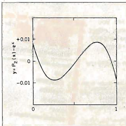
Figure 3: The approximation error in figure 2, magnified greatly for visibility.
