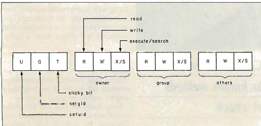
Figure 1: UNIX file permissions. Under the UNIX operating system, a user's ability to access a particular file is governed by the setting of 12 bits (four octal digits) associated with that file. The high-order 3 bits are the setuid , setgid , and "sticky" bits, respectively. The remaining 9 bits represent read, write, and execute/search permissions for owner, group, and others, respectively.
