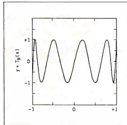
Figure 7: The Chebyshev polynomial of degree 9.
