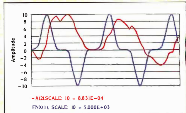
Figure C: A graph of displacement (X(2)) and driving force (FNx(T)) versus time for a system with Coulomb damping and nonlinear spring force.
