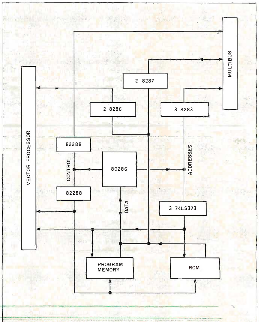
Figure 3: The configuration of the 80286, its program memory, and the Multibus interface.
