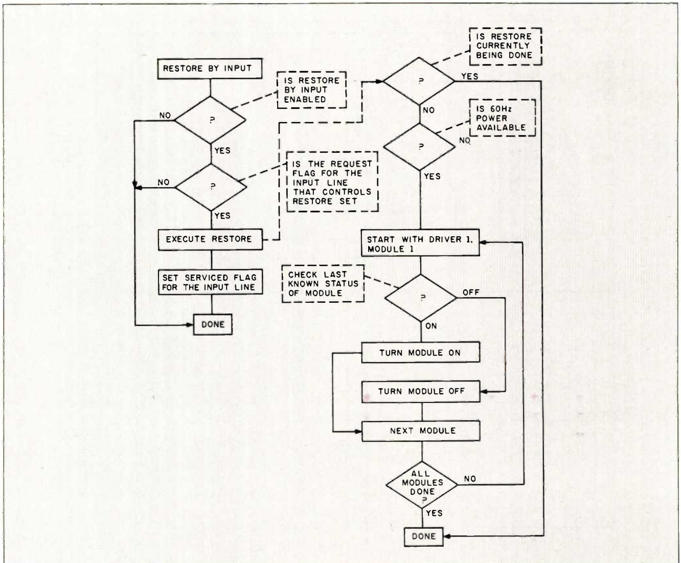
Figure 3: Restore Request Check flowchart.
