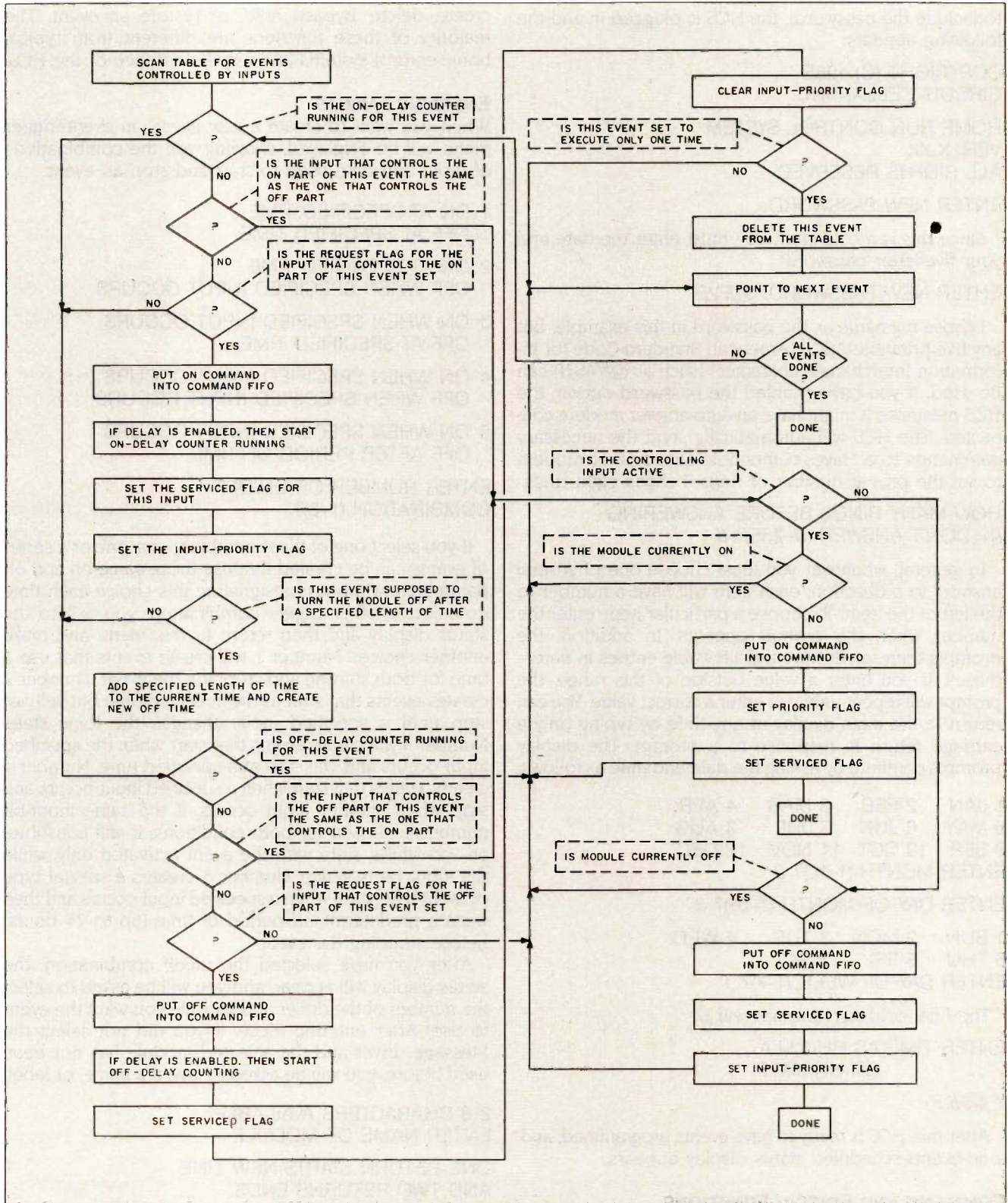
Figure 8: Scan for Input Events flowchart.
