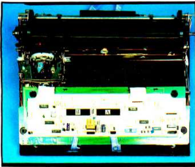
Photo 2: Bottom view of the component side of the keyboard assembly. Processors A and B are identified.
