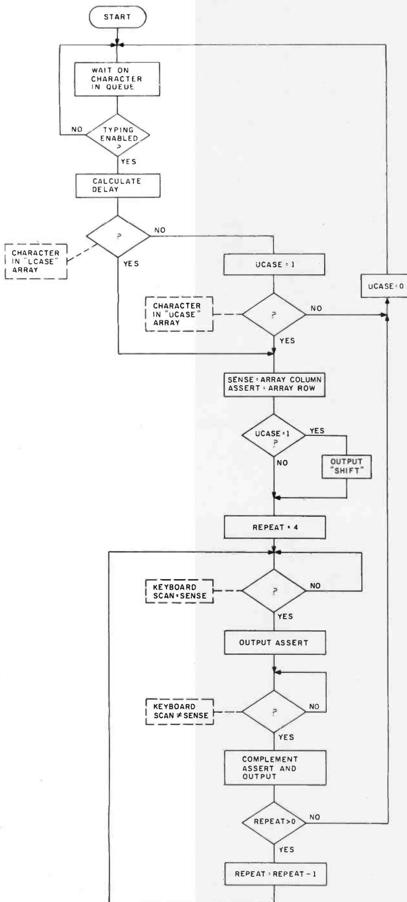
Figure 2: A flowchart of the controlling software as implemented in the C and Z80 assembler programs.
