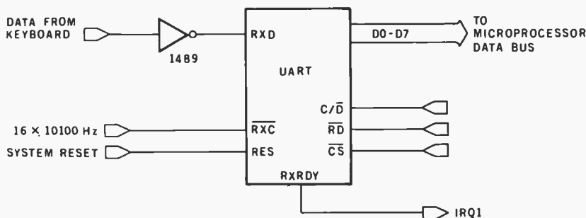
Figure 5: Interface circuit for using the IBM keyboard with another computer. The 1489-type inverting buffer changes the signal levels from the keyboard for use with the UART, which then changes the serial data to parallel format.
