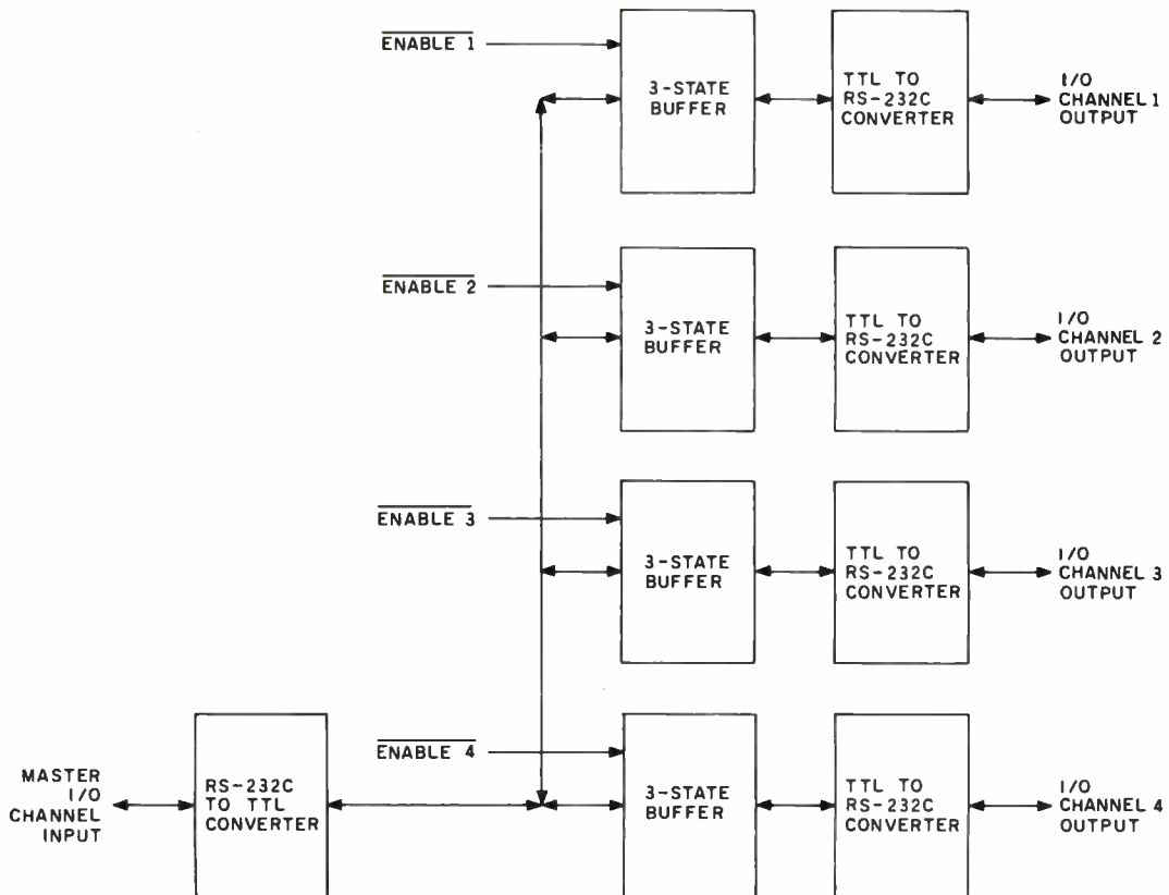
Figure 1a: Block diagram of a four-channel peripheral switch for RS-232C serial communication, which may be controlled via wired remote activation or code activation.
