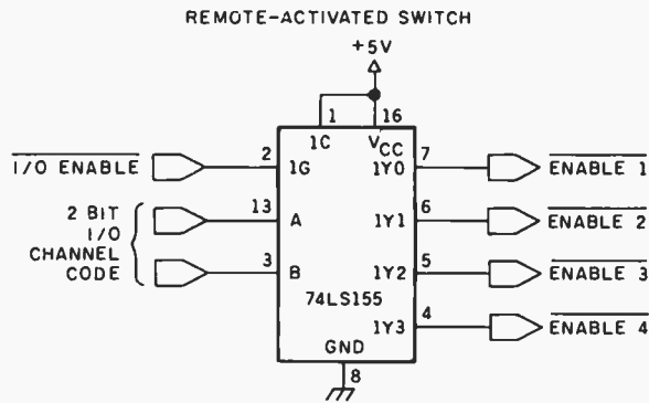
Figure 1b: Functional diagram of a 74LS155 two- to four-line demultiplexer as it would be connected in a peripheral switch using wired remote activation.
