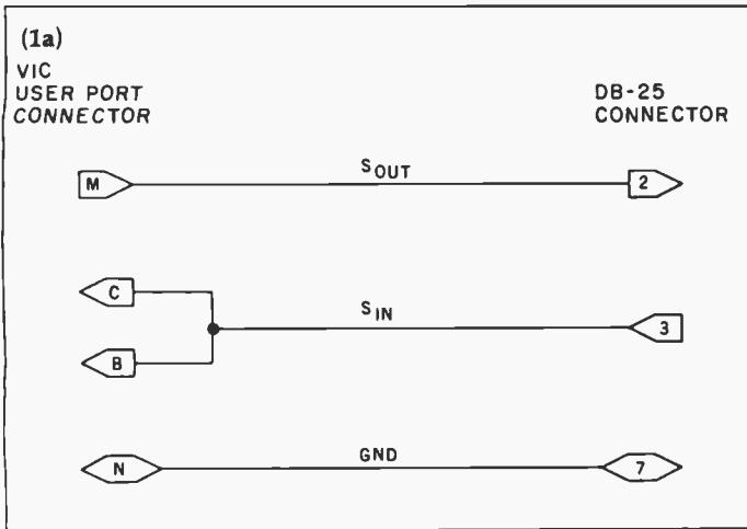
Figure 1: Schematic diagrams of connections between the VIC and other equipment. In figure 1a, the VIC is connected directly to a TTL-level compatible modem. Figure 1b shows the arrangement for connecting RS-232C-compatible DCE (data-communications equipment, such as a modem) to the VIC's serial port; figure 1c shows connections to DTE (data-terminal equipment, such as a printer or video terminal).
