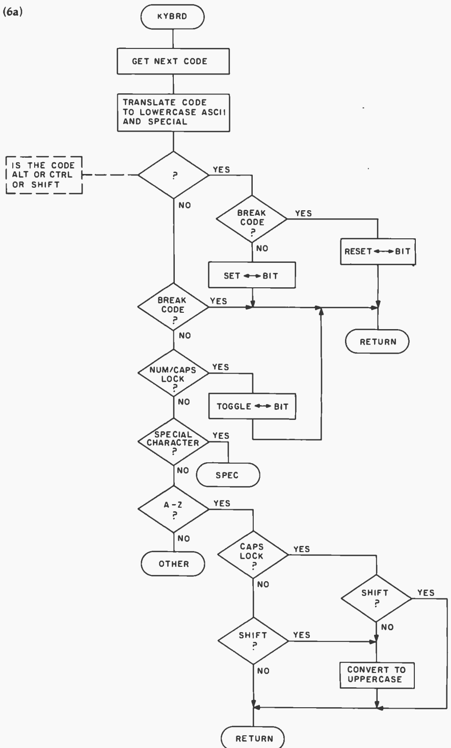
Figure 6: Flowchart of complete keyboard-encoder program shown in listing 2.
