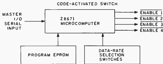
Figure 1c: Functional diagram of a Z8671 microcomputer chip (variant of a Zilog Z8) as it would be used to control a four-channel code-activated peripheral switch.
