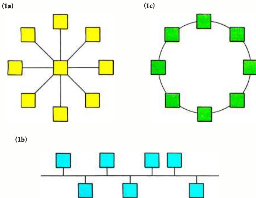
Figure 1: Popular network configurations. The star network (1a) is the most common of the early network types (such as the telephone system) and relies on the central node for control of operations. Bus configuration (1b), as used on the Ethernet and by cable television, allows nodes to be added or removed without impairing the network. The ring network (1c) circulates all messages in one direction and may pass tokens to specify which node may transmit; a failure of any node may interrupt network operation.
