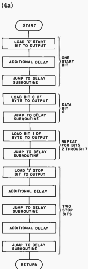
Figure 4a and b: Variable-bps-rate flow diagram showing a variable delay subroutine (4b) used to minimize storage space consumption. The main routine (4a) could be modified to transmit one stop bit if desired.
