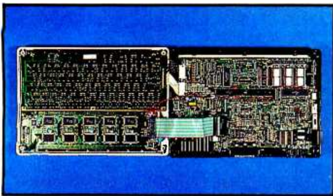
Photo 5: Inside the Model 100. On the right side are the undersides of the liquid-crystal display (top) and keyboard (bottom). The left side shows the main circuitry. The modem circuitry is in the upper left-hand corner. The random-access memory is in the lower left-hand corner. The 80C85 microprocessor is in the central part of the left side.
