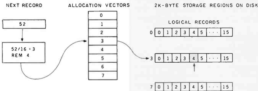
Figure 3: A diagram showing how the Winchester disk address is calculated. First, the value of the Next Record field is divided by 16. The resulting quotient points to one of eight allocation vectors, which in turn points to one of several 2K-byte regions on the disk. The remainder of the division points to one of the 16 logical records in each 2K-byte region.
