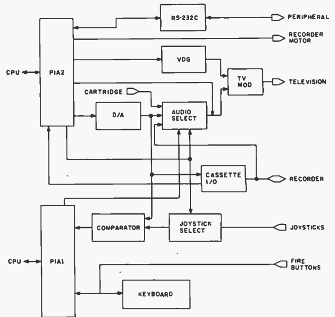
Figure 2: The TRS-80 Color Computer input/output system. The two PIAs are efficiently used to perform all of the I/O tasks needed by the Color Computer. The PIAs pass signals that are used for functions ranging from keyboard entry to cassette-recorder control to graphic-display control.
