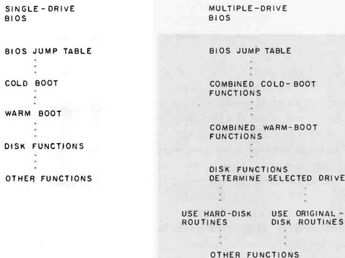
Figure 5: The combined BIOS structure.
