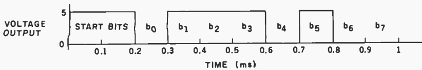
Figure 4: Diagram of the serial bit stream generated by the IBM PC keyboard when a key is pressed. The graph shows the voltage output (pin 2) versus time, starting when the C key (code 46 decimal, or 00101110 binary) is pressed. The voltage levels are TTL-compatible. In the absence of transmission, the keyboard sends a 0-V level. Two +5-V (high) "start bits" define the start of a character. Eight bits follow, each lasting 0.1 ms, except for the last, which is slightly shorter.
