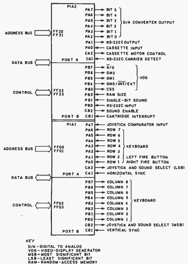
Figure 3: The PIA pin assignments. All available connections to the two PIAs are used, in some cases for more than one purpose. The great flexibility of the MC6821 makes this efficiency possible.
