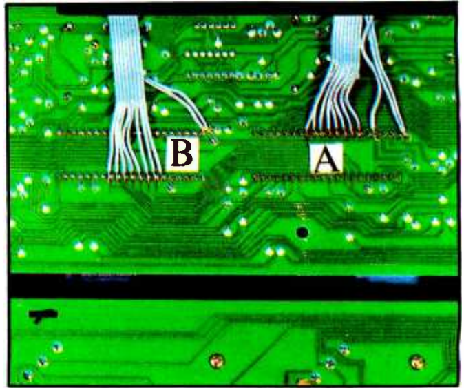
Photo 3: View of the printed-circuit side of the Praxis processor board. Note where the flat ribbon cables are connected to the A and B processors. Wires from Processor A connect to the output side of the parallel port. The lower board is the keyboard.
