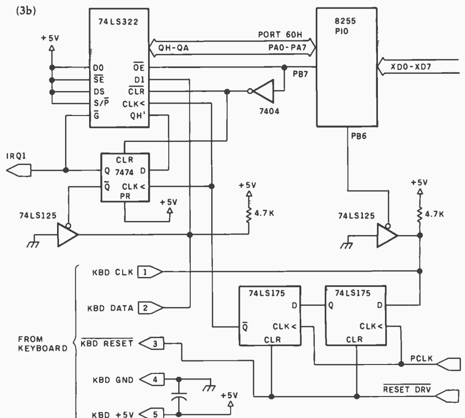
Figure 3: Interface circuitry used by IBM. Figure 3a is a partial diagram of the transmission circuitry used by IBM in its keyboard, as shown on page D-12 of the IBM Personal Computer Technical Reference Manual. The Personal Computer's keyboard input-port interface, from page D-10 of the manual, is shown in figure 3b.
