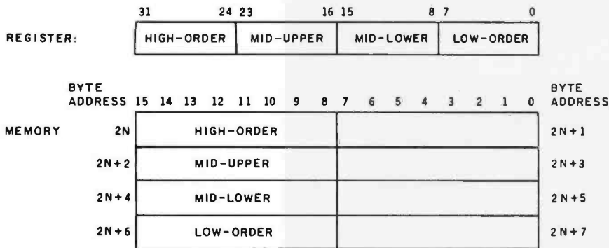
Figure 1: Moving data from a 32-bit register to memory using the MOVEP instruction. Bytes from the register are stored in every other memory byte. The instruction takes 24 clock cycles to execute.
