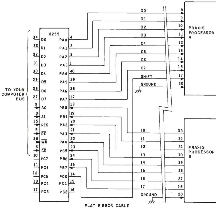
Figure 1: The interconnection between an Intel 8255 parallel-port chip and the Praxis microprocessors.
