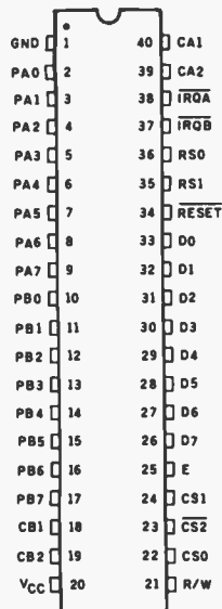
Figure 1: The peripheral interface adapter (MC6821) provides a flexible general-purpose interface between any of the 6800 series microprocessors and the outside world.
