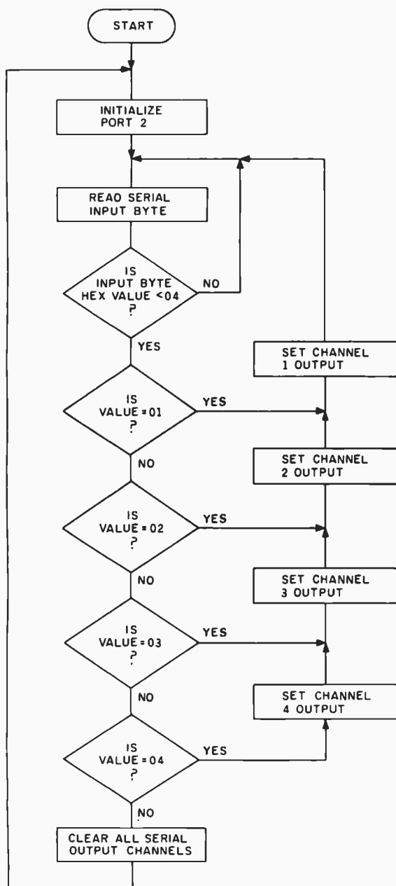
Figure 3: Flowchart of a Z8-BASIC/Debug program to control the four-channel code-activated switch at low data rates.
