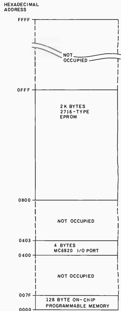
Figure 2: Memory map of the module's address space. Unoccupied gaps are due to the simple decoding method that uses some address lines to directly enable the peripheral integrated circuits.
