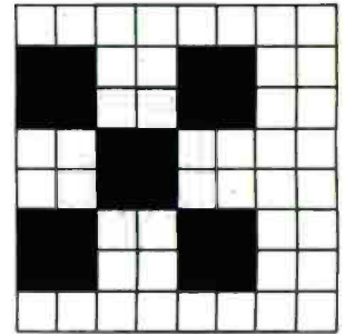
Figure 5: Inverse video character. By having all the bits in the bit pairs on and printing the character as an inverse video character you can obtain the color in register 3.
