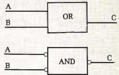
Figure 9 (OR circuit)
