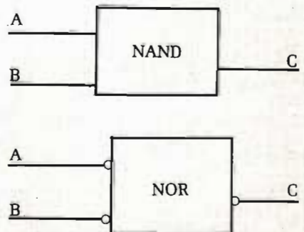
Figure 10 [NAND circuit]
