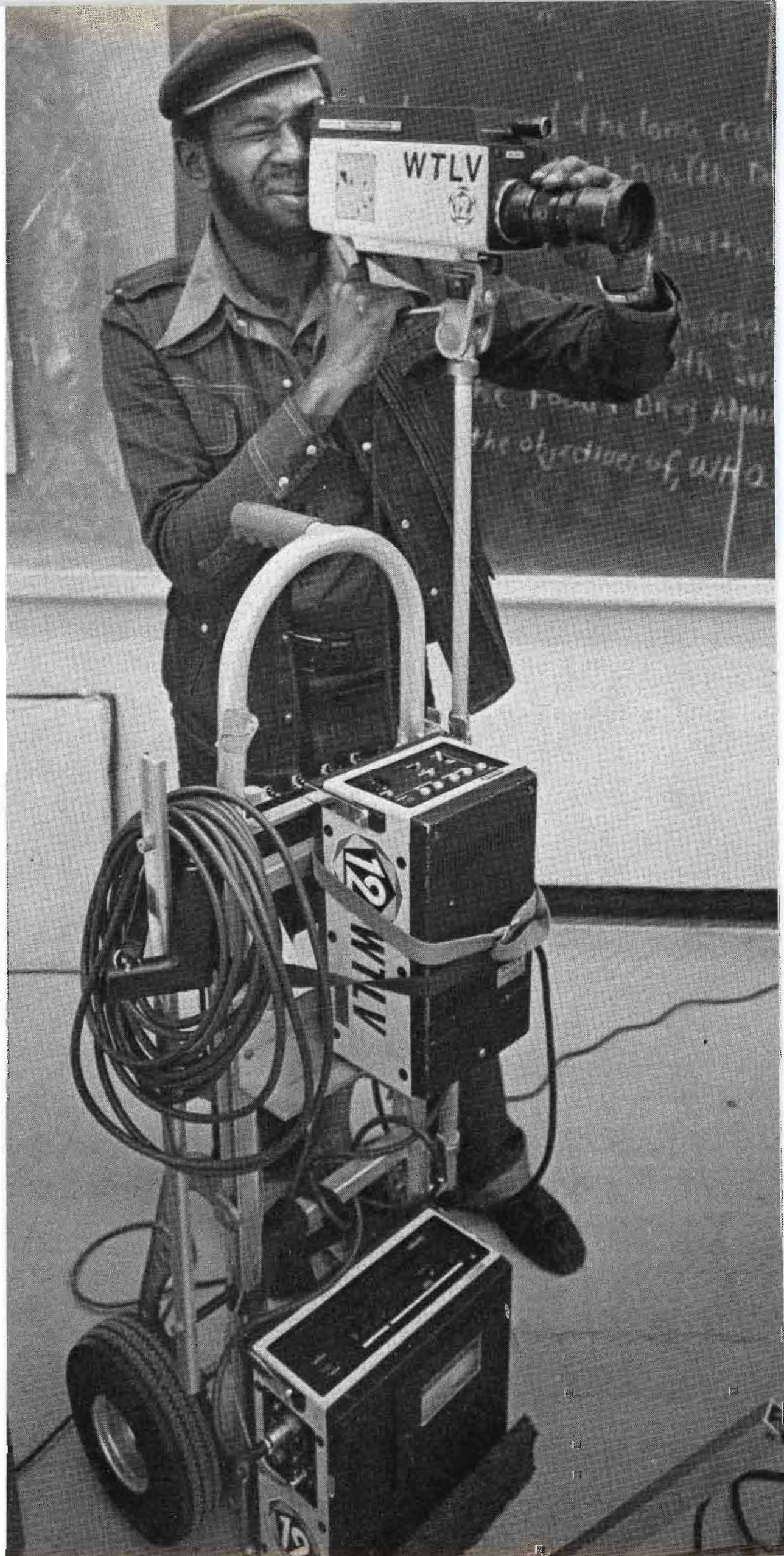
This golf cart-like apparatus is used to transport ENG equipment from the van into the news scene. Below the camera is the CCU. The 3/4-inch tape machine is at the bottom.
