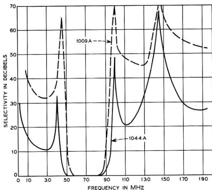
Fig. 10—IF selectivity.
