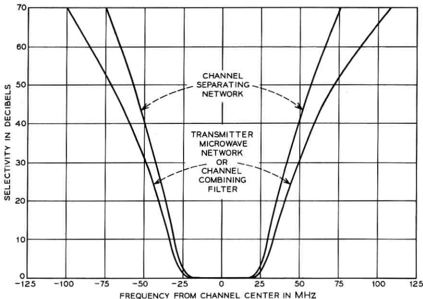
Fig. 9—RF selectivity.
