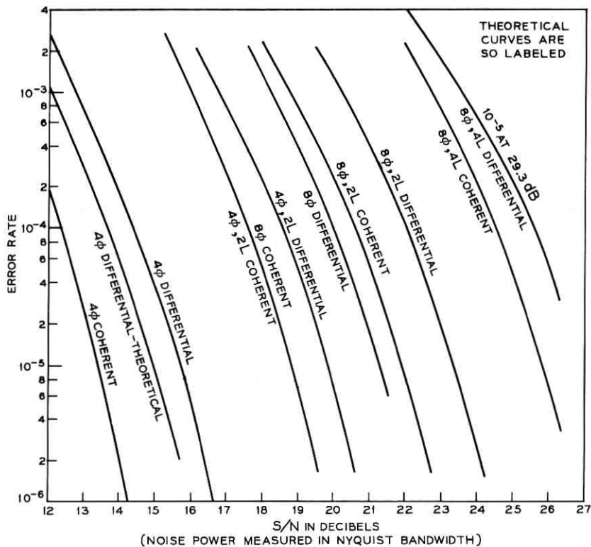
Fig. 10—Performance curves.
