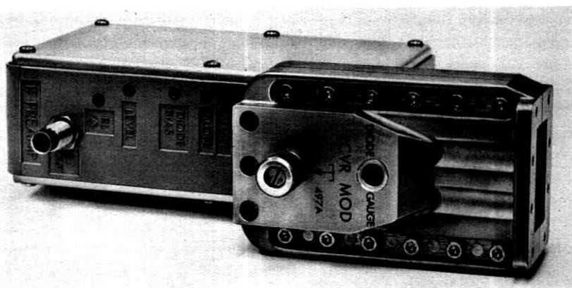
Fig. 3—Receiver modulator.
