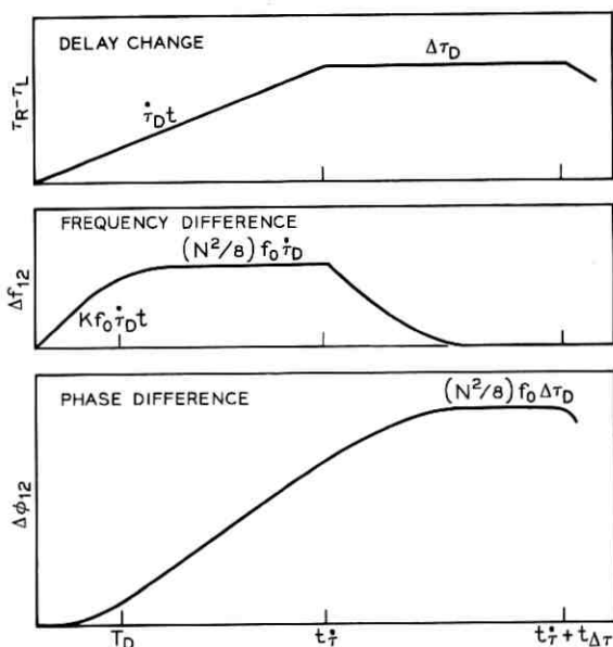
Fig. 2—Response of dumbell to delay change.
