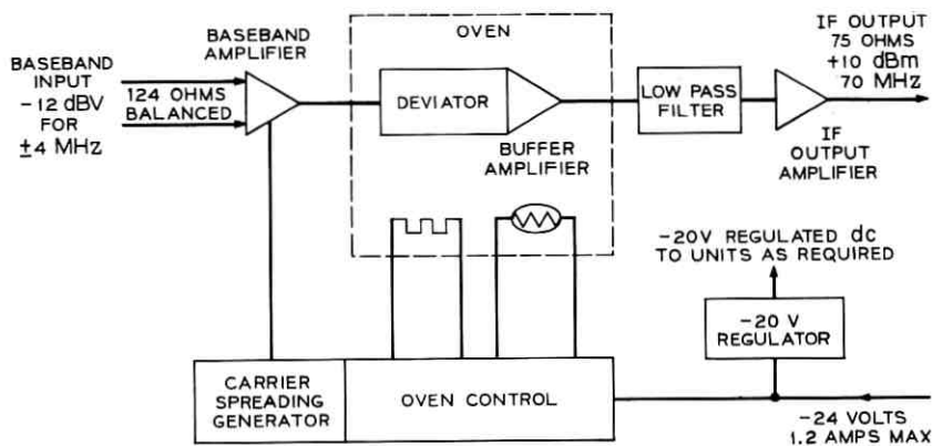
Fig. 2—Block diagram of 4A FM transmitter.
