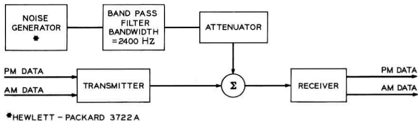
Fig. 9—Experimental configuration.
