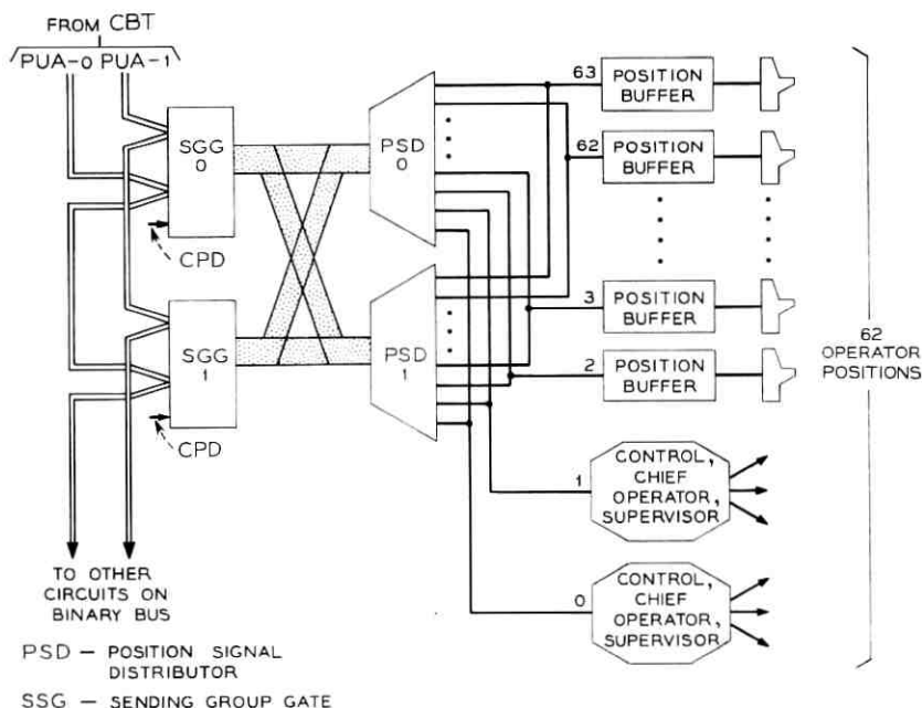
Fig. 20—Local subsystem—sending.
