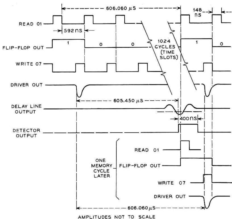
Fig. 6—Delay-line loop timing.
