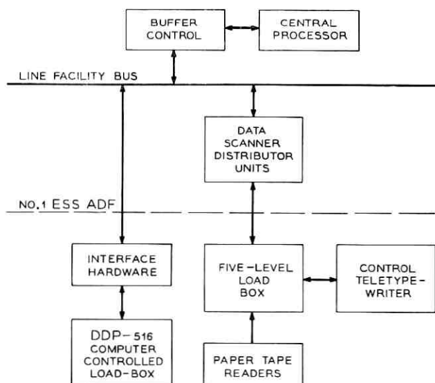
Fig. 12—Load box facilities used in testing the No. 1 ESS ADF system.
