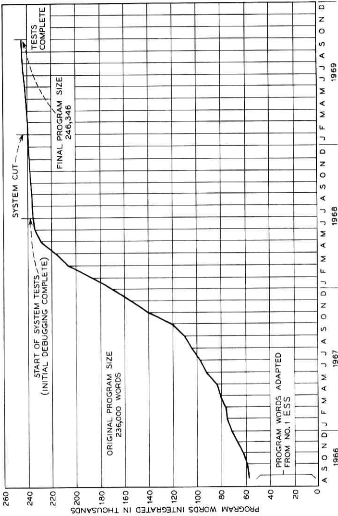
Fig. 1—No. 1 ESS ADF program integration.
