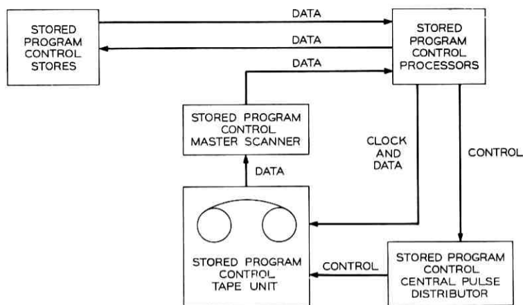
Fig. 11—Block diagram of program tape unit.
