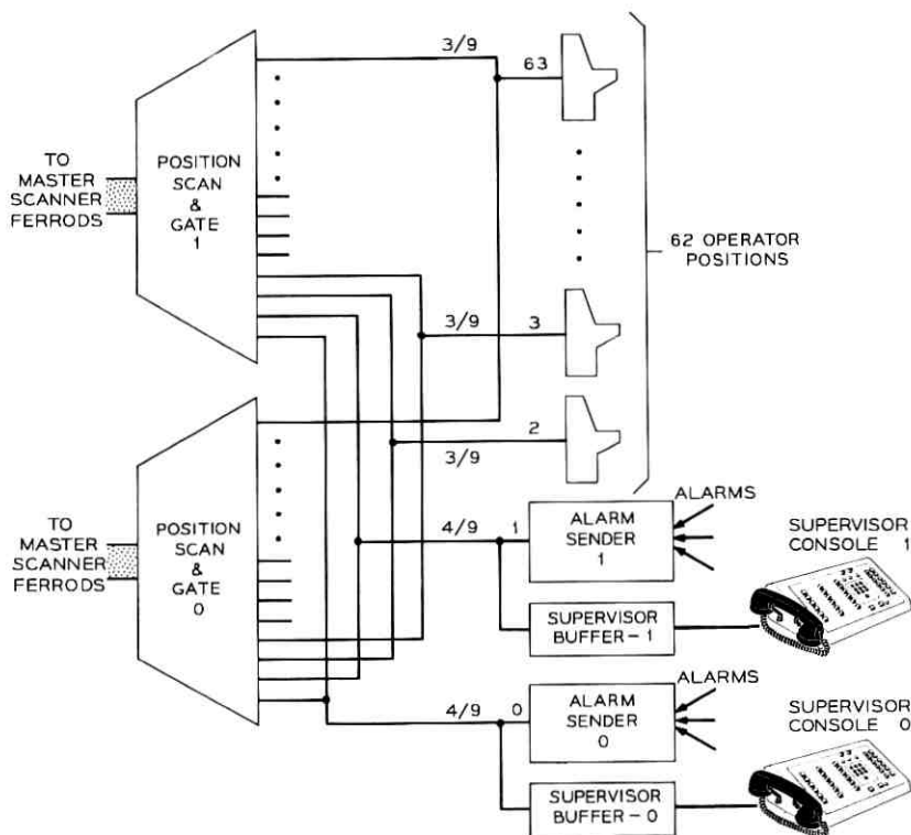
Fig. 23—Local subsystem—receiving.
