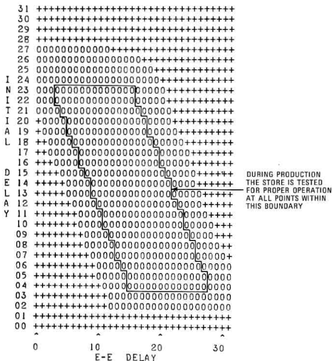
Fig. 22—Strobe window.
