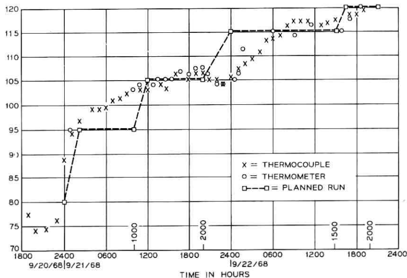
Fig. 21—Schedule and reading for temperature tests.
