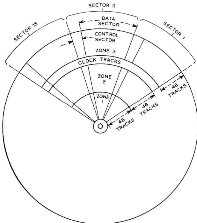
Fig. 1—Disk surface geometry as determined by word clock.
