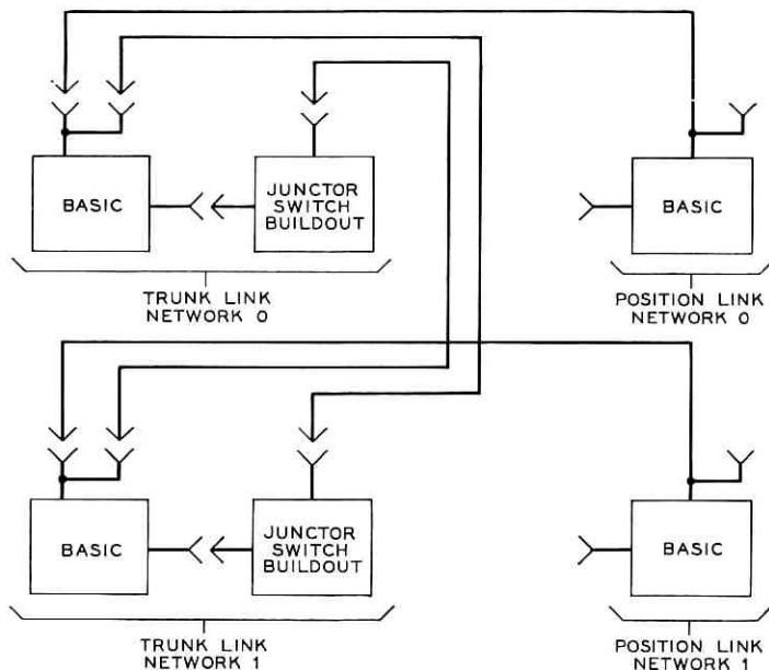
Fig. 9—Two-network configuration.
