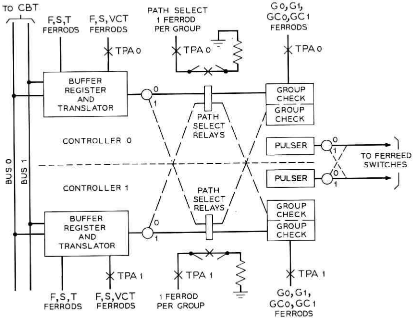
Fig. 12—Network controllers.
