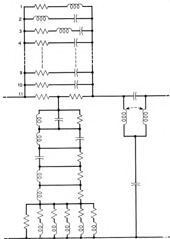
Fig. 19 — Schematic of network equalizer.
