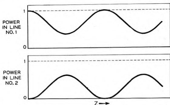
Fig. 3 — Incomplete power transfer resulting from coupling two lines having different phase velocities
