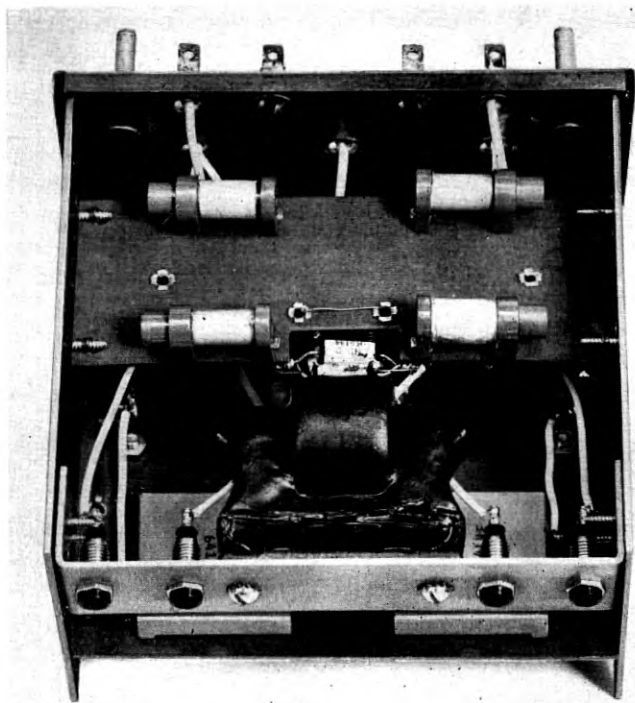
Fig. 25 — Photograph of output network.
