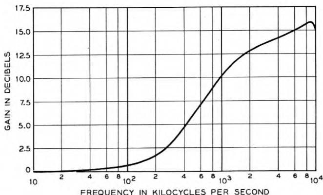
Fig. 17 — Gain characteristic of input network.
