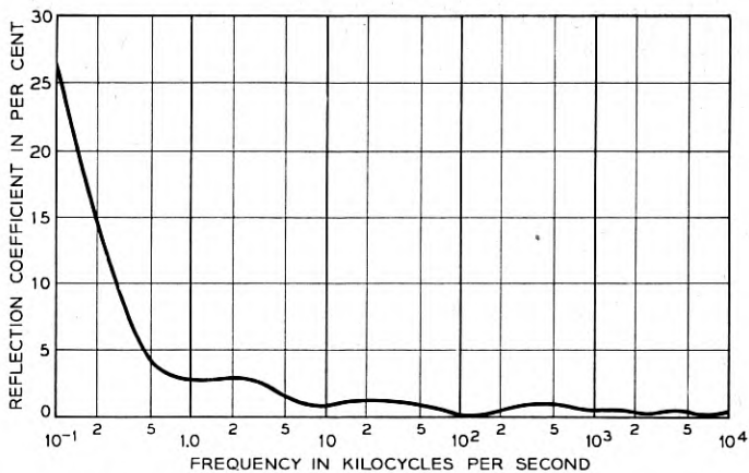
Fig. 7 — Reflection coefficient of network against cable impedance.
