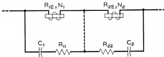
Fig. 18 — Series relays with one RC network.
