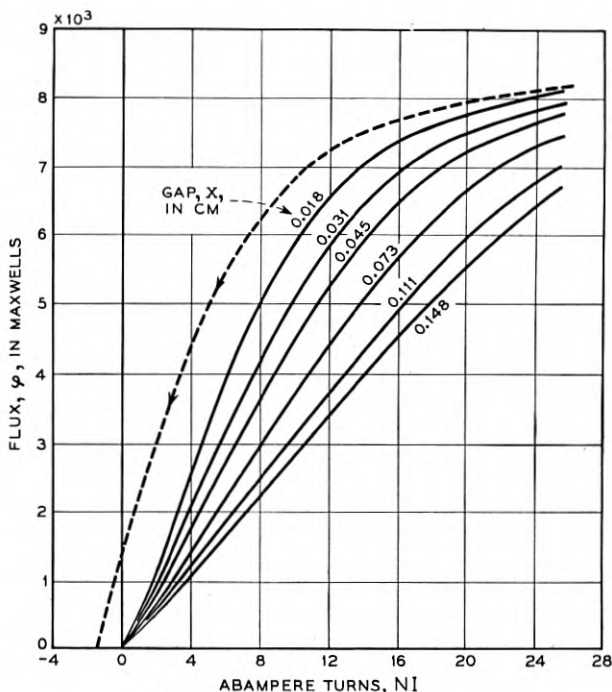
Fig. 1 — Magnetization curves.
