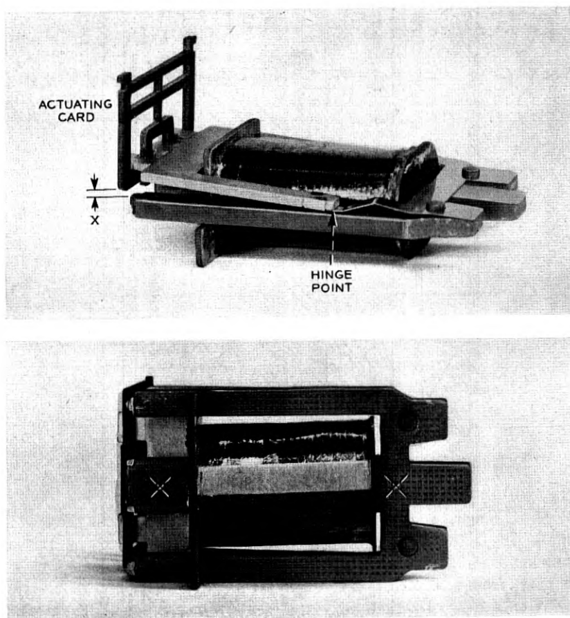
Fig. 2 — Magnetic parts, coil, and actuating card of AJ relay.
