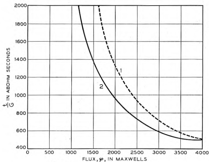
Fig. 3 — Release time versus flux.
