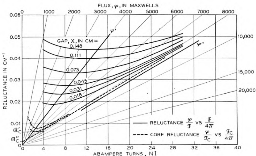
Fig. 3 — Reluctance curves.
