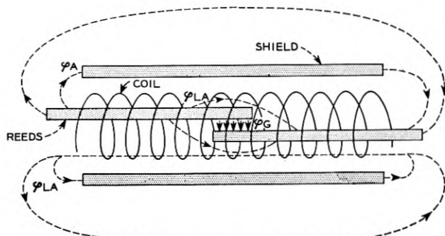
Fig. 24 — Magnetic field of a reed relay.
