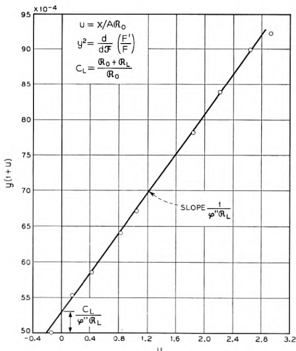
Fig. 14 — Evaluation of saturation flux \varphi'' and leakage reluctance \mathcal{R}_L from pull characteristics.
