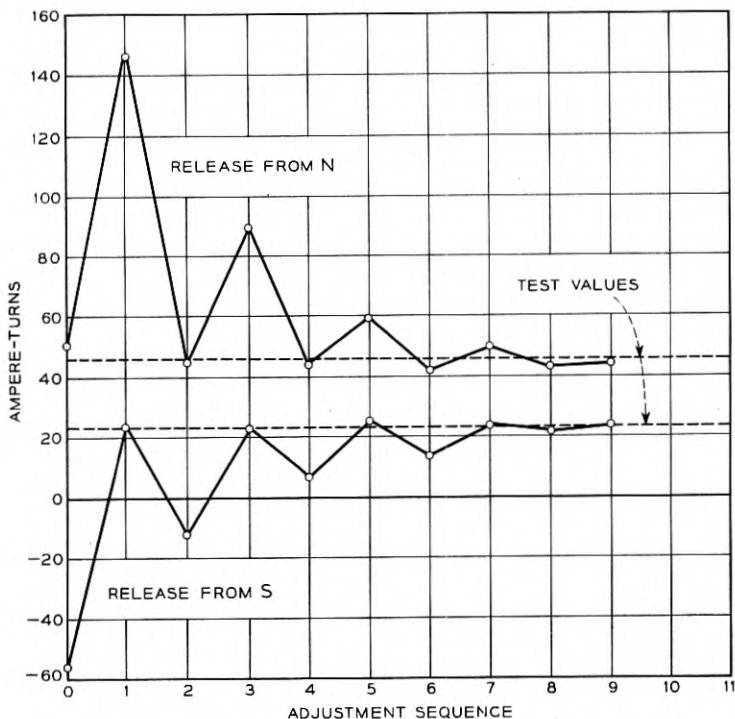
Fig.13 — Sequence of sensitivity values obtained in adjustment.
