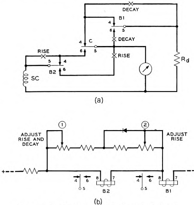
Fig. 10 — Final schematic of basic contact circuit.
