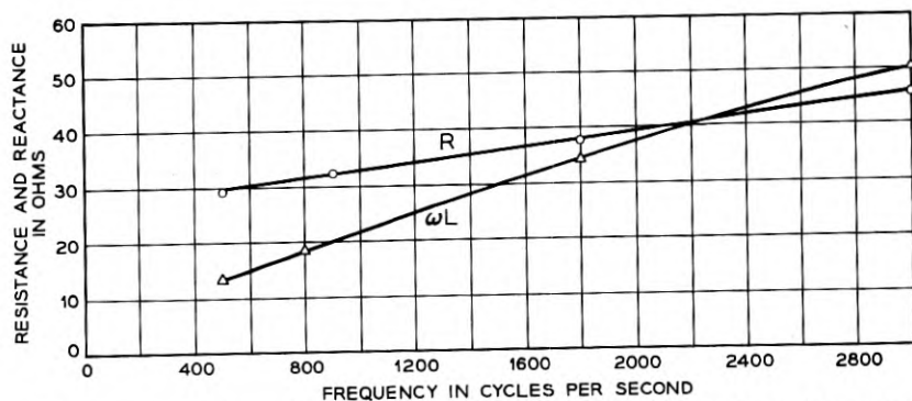
Fig. 8 — Resistive and inductive components of impedance for a large area cathode tube as a function of frequency. I_{dc} = 25 mm.
