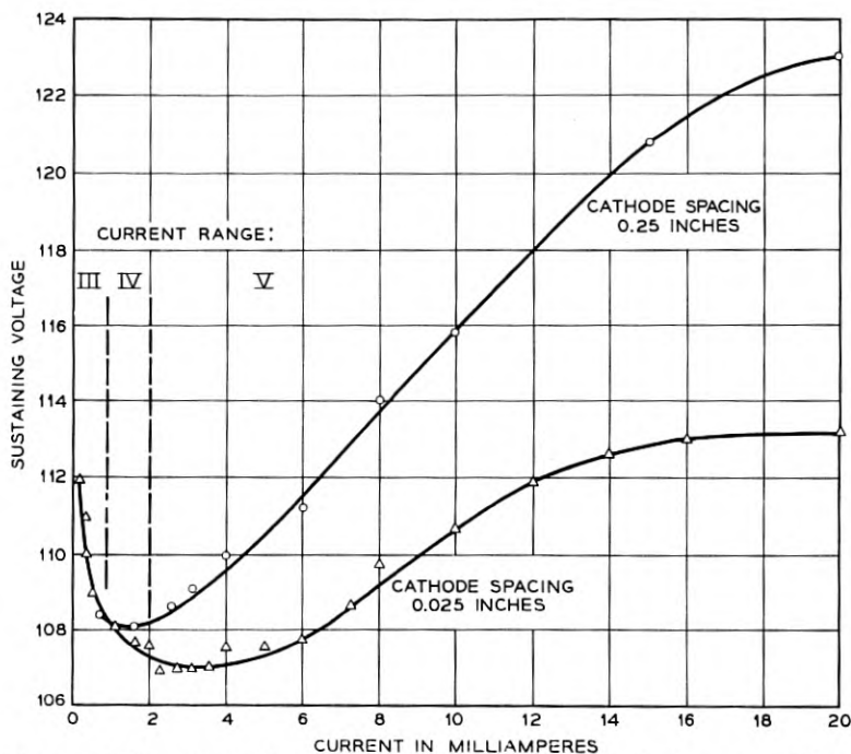
Fig. 2 — Volt-ampere characteristic of parallel plane cathodes at two different spacings.
