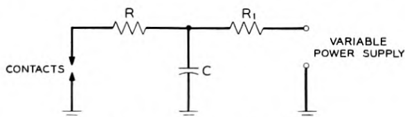
Fig. 1 — Contact Circuit.
