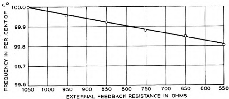
Fig. 10 — Effect of feedback on frequency.
