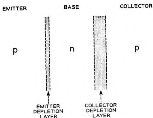
Fig. 1 — p-n-p transistor.
