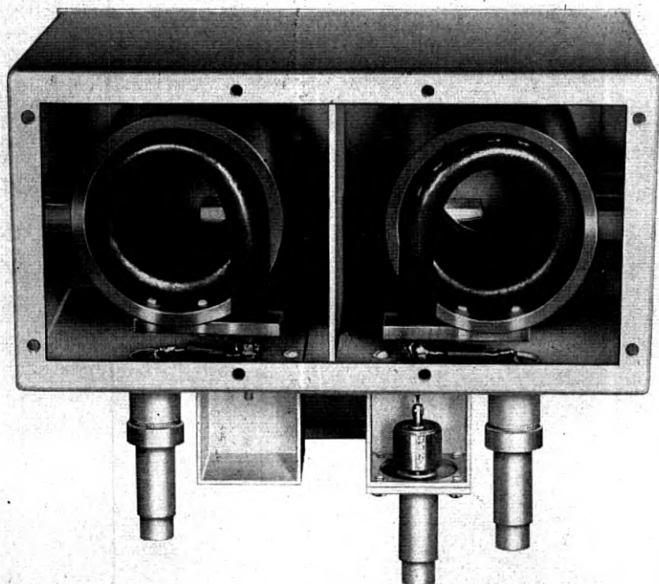
Fig. V-12.—Unbalanced to balanced coaxial transformer for feeding the 65 mc signal to the transmitting converter.
