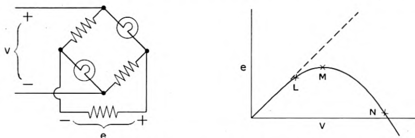
Fig. 17—D-C characteristics of a lamp bridge.
