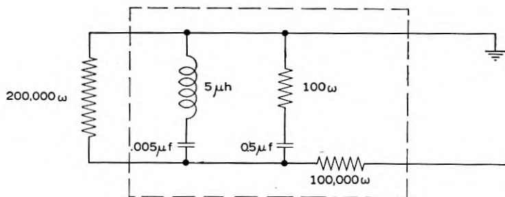
Fig. 25—Configuration of auxiliary filter.
