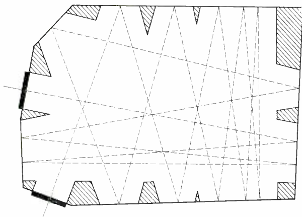
Fig. 4 — Configuration of a double wedge, 500-microsecond delay line.
