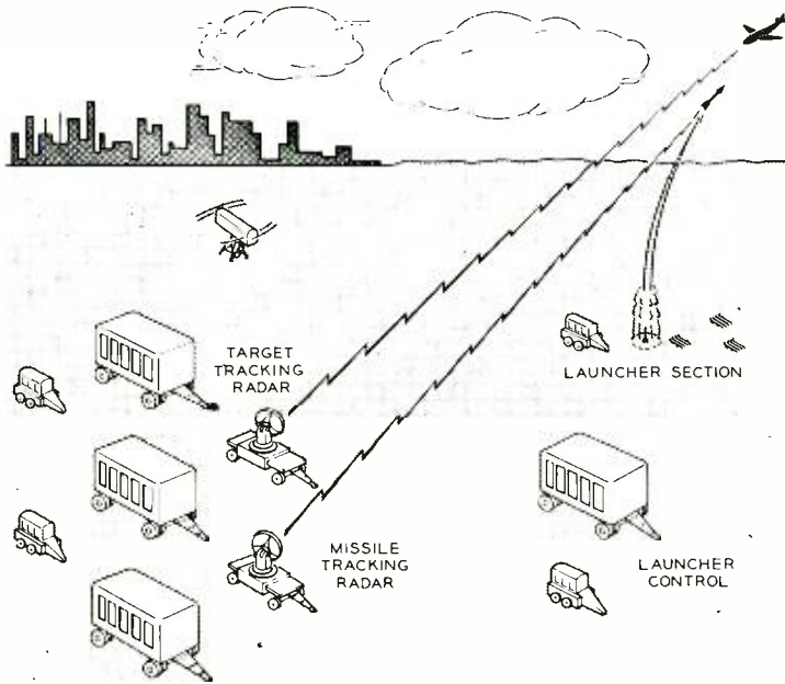
Fig. 1—The Nike missile system.
