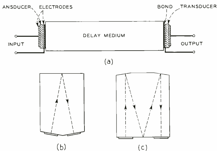
Fig. 1—Typical simple delay line configurations: (a) rod type; (b) single reflection type; (c) triple reflection type.
