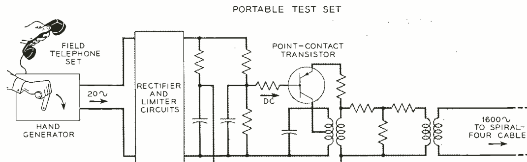
Fig. 1 — Portable telephone and test set signaling arrangement. Transistor circuit supplies 1,600 cps tone to cable.
