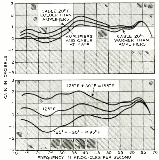
Fig. 4 — (a) Gain-frequency characteristics of 200-mile system, showing changes when cable is colder or warmer than amplifiers; (b) characteristics for hot-weather operation on the same system.
