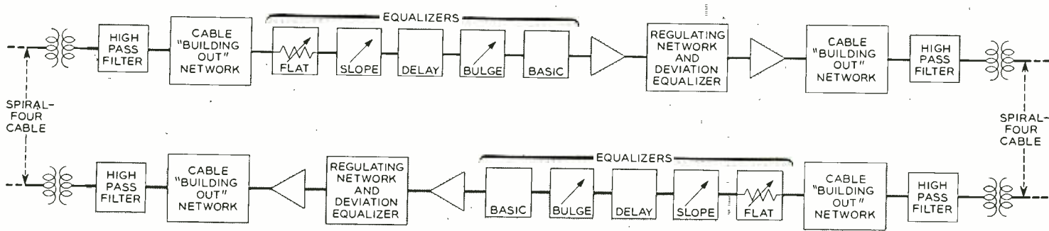
Fig. 5 — Block diagram of the carrier frequency transmission paths of the AN/TCC-8 telephone repeater.
