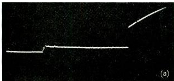
Fig. 1 — (a) Oscillogram of a sustained arc on break followed by an open circuit. Starting from the left, the contacts are closed at first and the trace is a horizontal line at zero voltage. The contacts then open into an arc at 15 volts which lasts for about 300 microseconds. When the arc goes out, the voltage jumps to a new value, then charges up more slowly because of the current from the external source. (b) “Showering” on break followed by a glow discharge. After the portion of the trace at zero voltage, there is a region of rapid charge-ups and breakdowns lasting for about 30 microseconds. This is followed by a steady glow discharge at 300 volts lasting for about 70 microseconds. When the glow discharge goes out, the voltage begins to fall as the capacitance discharges through the power source, which supplies only 50 volts.
