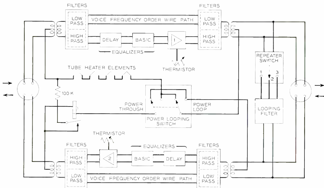
Fig. 2 — Block diagram of AN/TCC-11 unattended repeater
