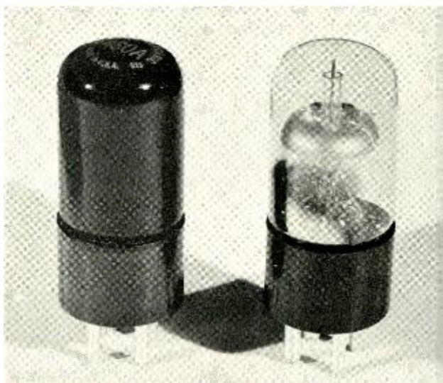
The new Western Electric 430A tube with and without opaque coating.
