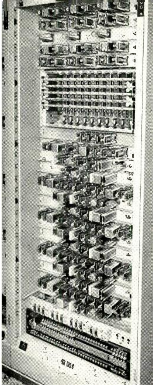
Fig. 2—Lower part of trunk bay showing one ringing switch.
