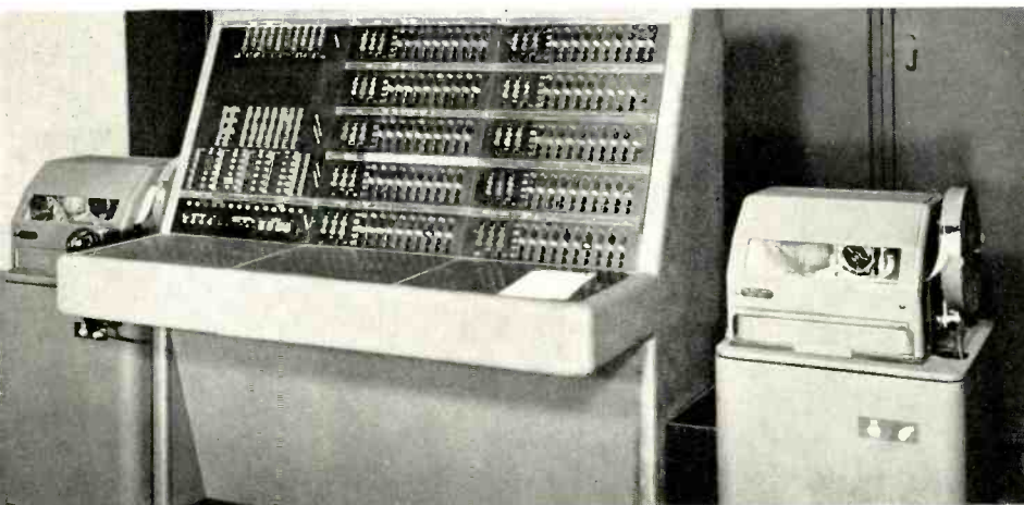
Fig. 6—Control board and intercept typing reperforators.
