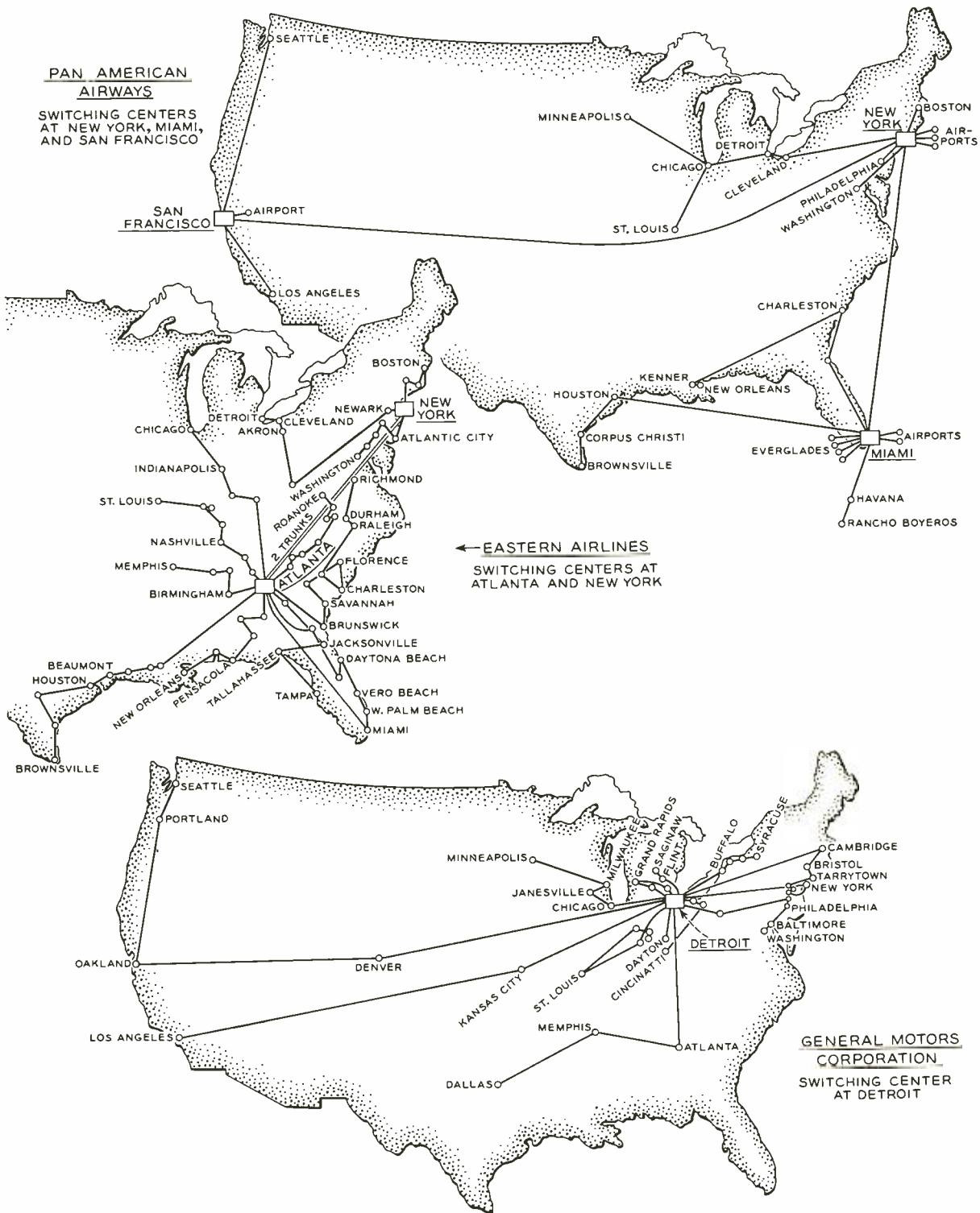
Fig. 2—Circuit maps of the 81-C-1 teletypewriter switching system installed for the Pan American Airways, the Eastern Air Lines, and the General Motors Corporation.
