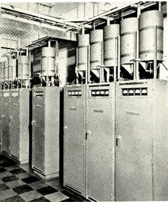
Fig. 2—Tuned cavities mounted above the transmitters in Chicago to attenuate intermodulation products resulting from carrier picked up from adjacent antennas.
