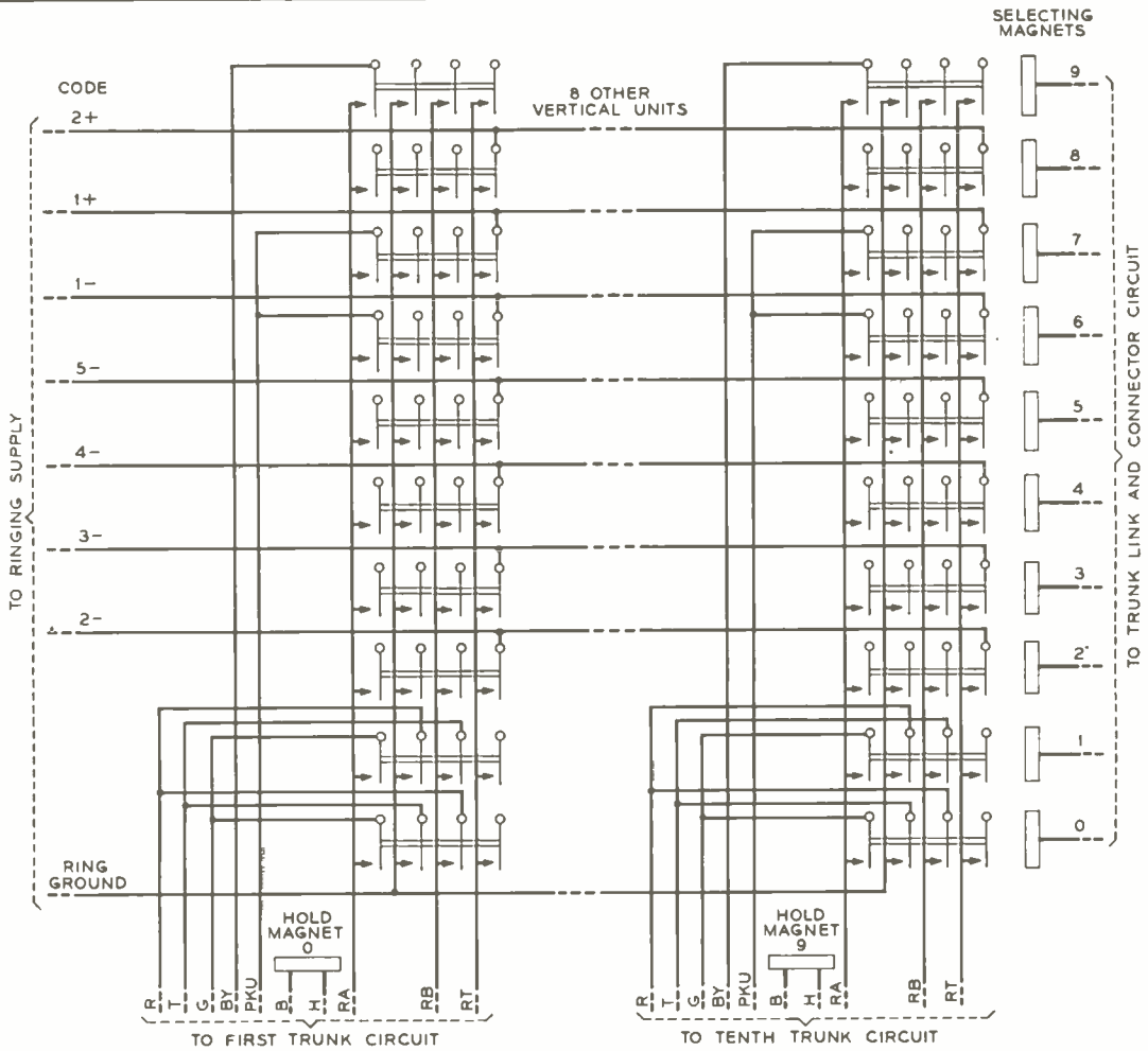
Fig. 3—Simplified schematic of ring circuit in a No. 5 crossbar office.
