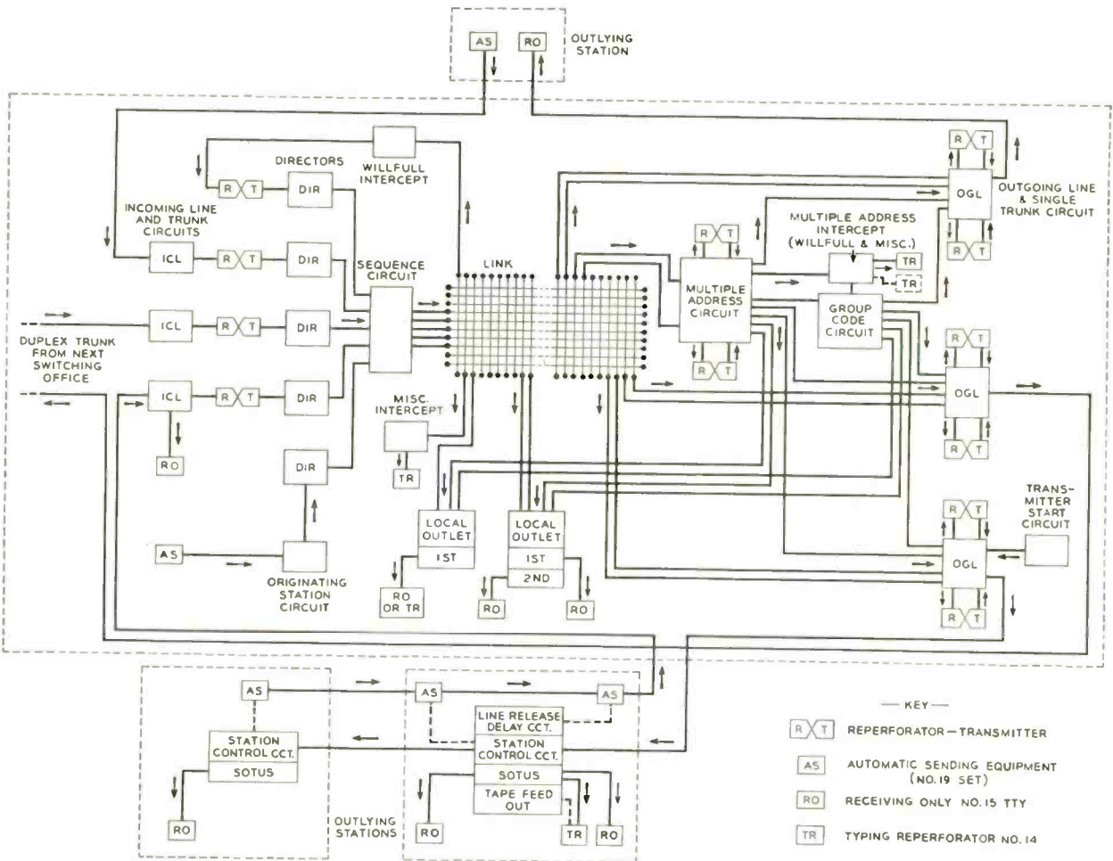
Fig. 3—Block schematic for the 81-C-1 system.
