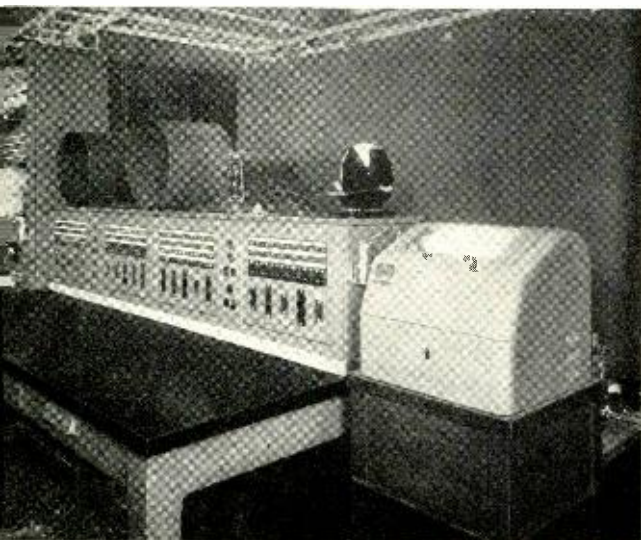
Fig. 8—Test bench and turret with monitoring teletypewriter at right, as installed at Pan American Airways.
