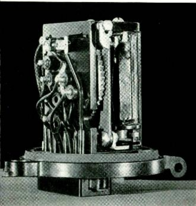
The transmitter with cover removed to show the operating magnets and the ratchet wheel provided for carrying the contacts
