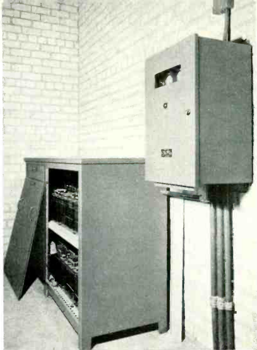
The alarm battery and automatic charger are in a room adjacent to the control center
