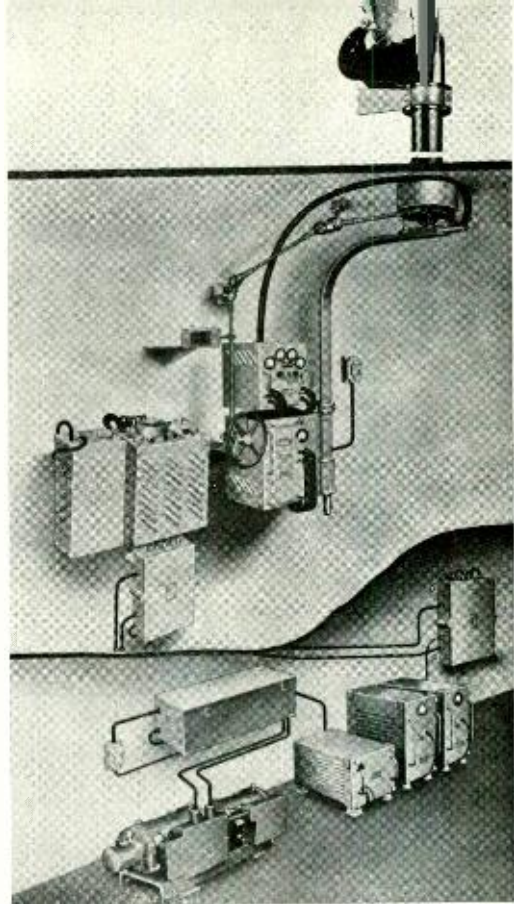
Typical arrangement of SJ radar apparatus in a submarine
