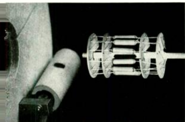
The rods to be glazed are mounted in four slotted disks on an extension of the shaft of a motor that rotates at a slow speed
