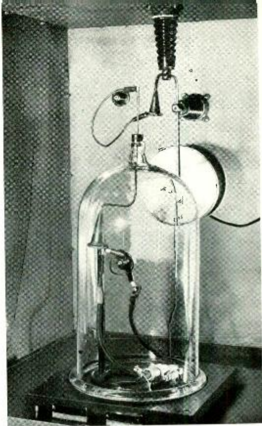
Interior of test cabinet showing bell jar used for tests at reduced air pressures
