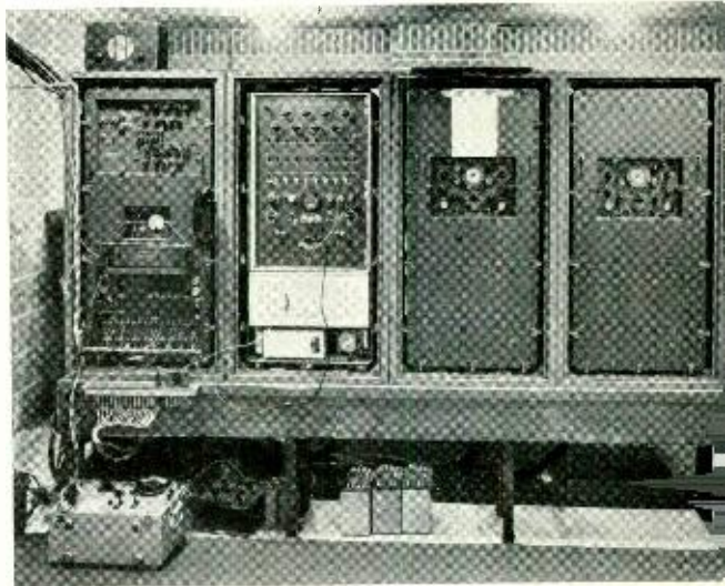
Equipment panels at the Barnstable terminal of the Barnstable-Nantucket microwave radio link
