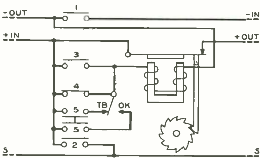
Simplified schematic of transmitter circuits before an alarm has been turned in, above, and after operating magnet has released following the first operation
