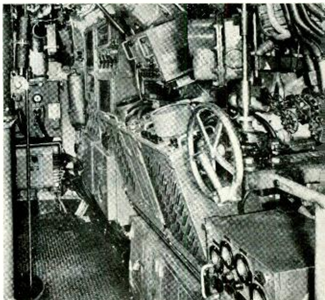
Interior of conning tower looking aft: main control unit at the lower right; transmitter receiver center left; hand wheel for training antenna, center right
