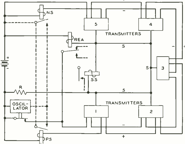
Simplified schematic of alarm circuit
