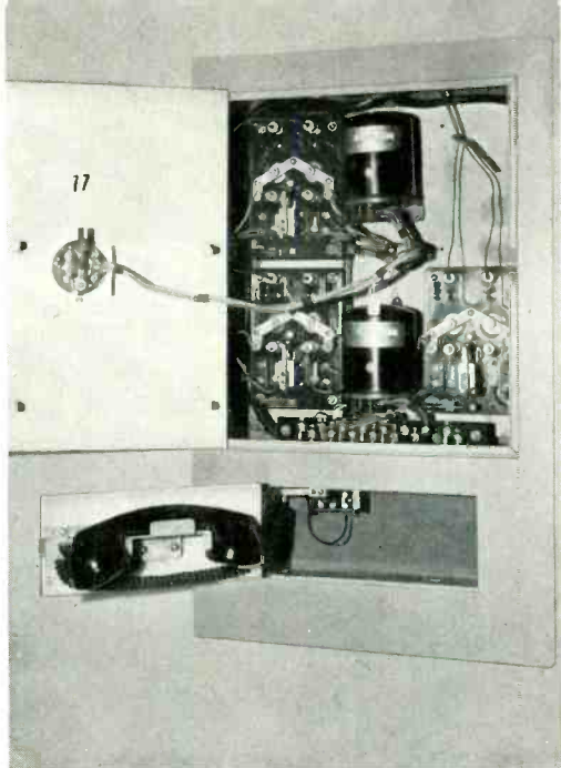
A fire alarm installation in one of the stairwells of the Murray Hill Building
