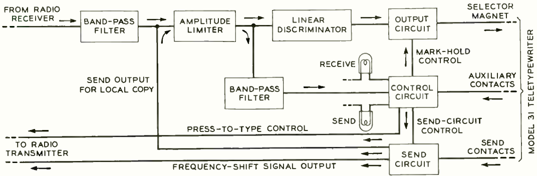
Block schematic of a telegraph terminal
