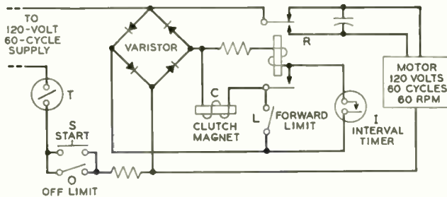
Circuit diagram of the automatic glazing machine. Pushing the button S energizes the magnetic clutch C and moves the thermistor units into the furnace until stopped by the limit switch L. At the end of the time interval chosen the timer I re-energizes the clutch and reverses the motor
