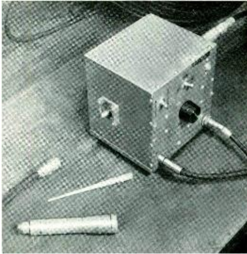
Fig. 3—The shielded voltmeter includes a short section of air-dielectric coaxial. This is larger in diameter than the cable under test, and five-inch tapered coaxial lines are used for the inter-connection
