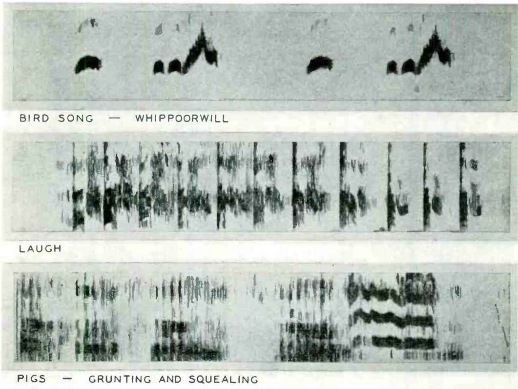
Fig. 6—Various sounds as recorded in visible speech
