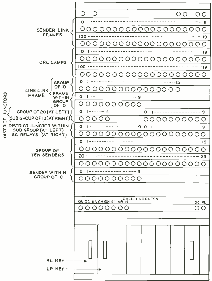
Fig. 6—Lamp arrangements in trouble indicator
