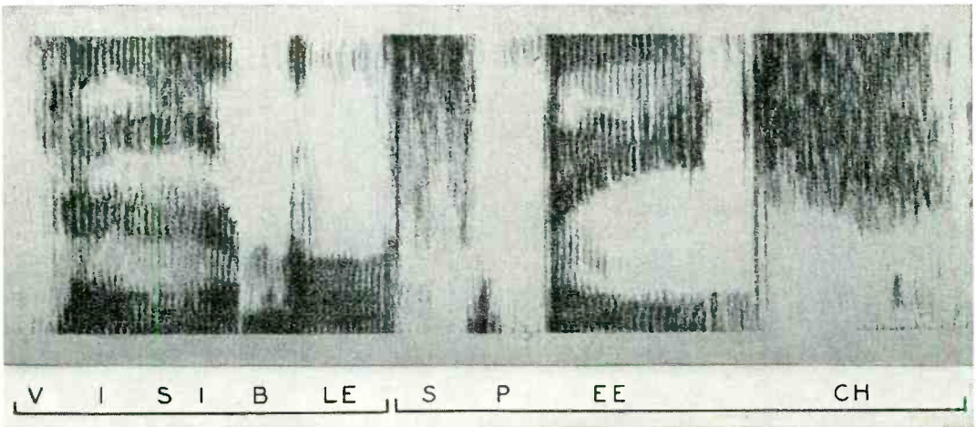
Fig. 3—The words "Visible Speech" as they would appear in visible speech
