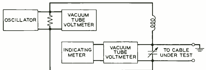
Fig. 5—Schematic circuit of Boonton 170A Q-meter
