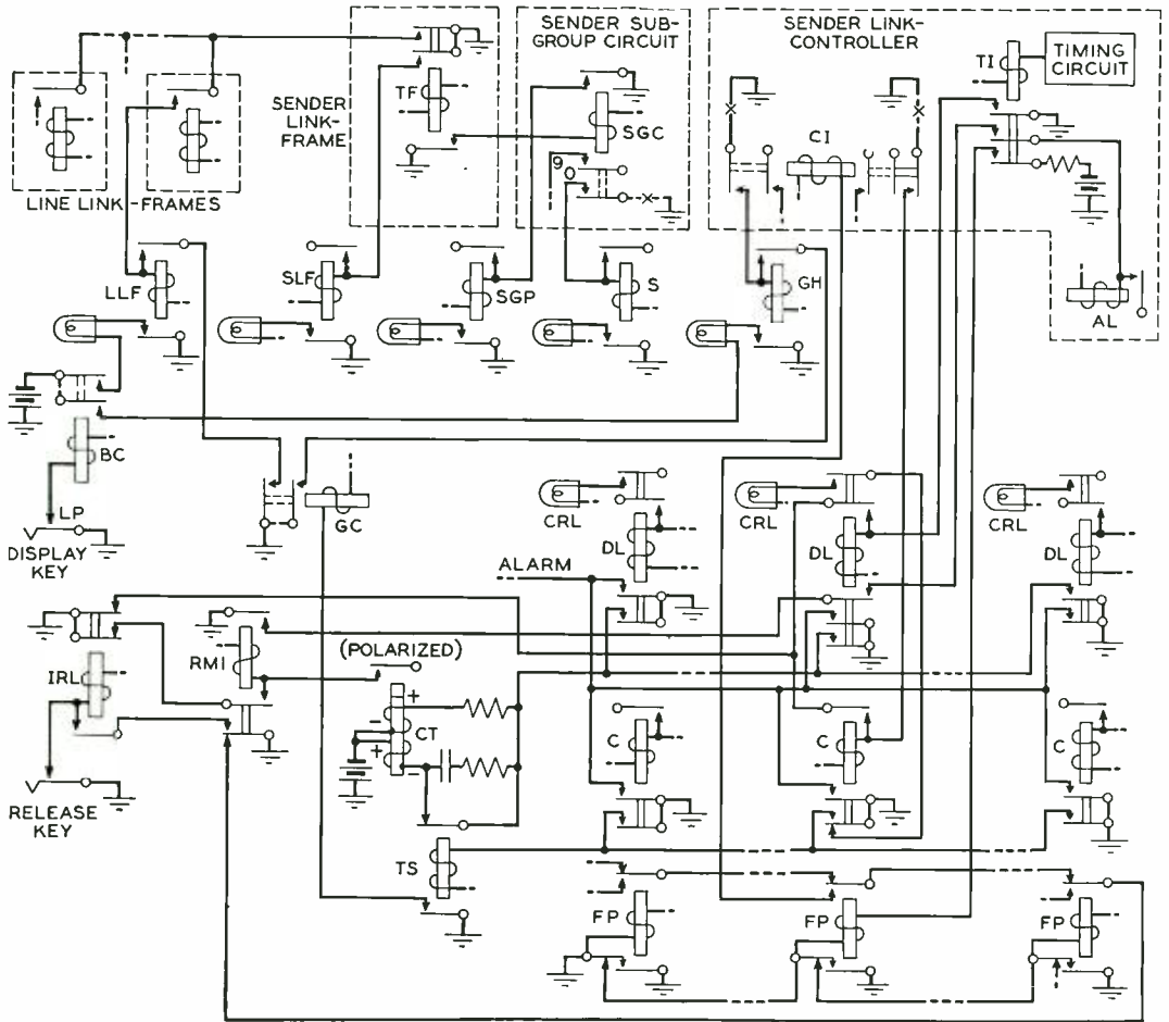
Fig. 3—Simplified schematic of some of the principal circuits of the trouble indicator
