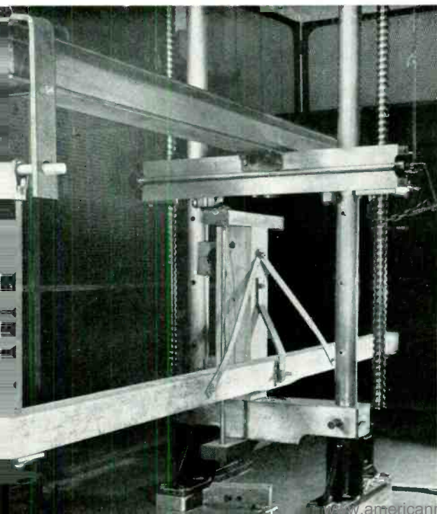
Fig. 3 (below, right)—The break occurs at one of the inner pinholes of the crossarm where the fiber stress set up is greatest
