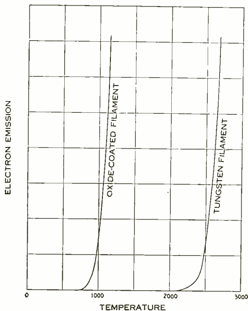
Electron emission and temperature
