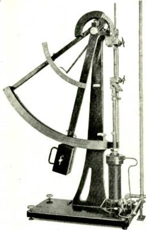
The Schopper tester for light tensile tests such as cable-paper and materials for transmitter diaphragms
