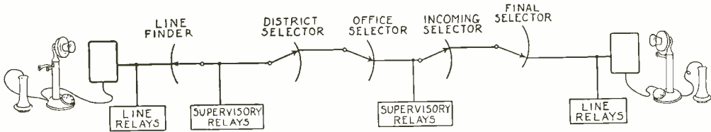
How the circuit stands during conversation
