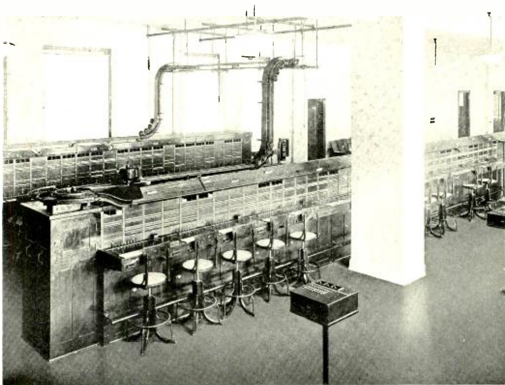
The mechanical system as installed at Omaha. In the foreground, the recording board; behind it, a part of the outward line board. Note the overhead crossing
