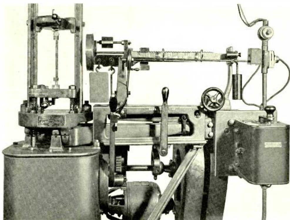
A 10,000-pound tensile testing-machine. Force exerted on the sample (left) is measured by its reaction on the scale beam
