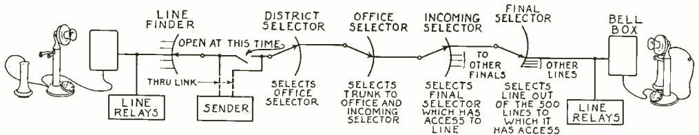
How the connection looks while the called subscriber's bell is being rung
