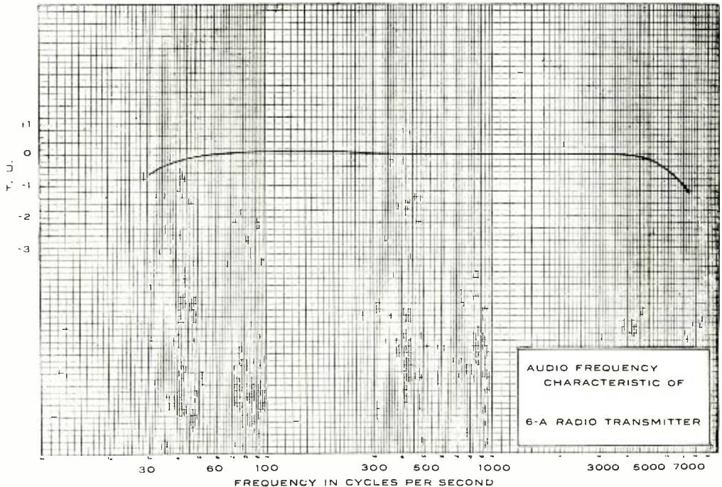
Audio-frequency characteristic of the 6-A Radio Transmitter
