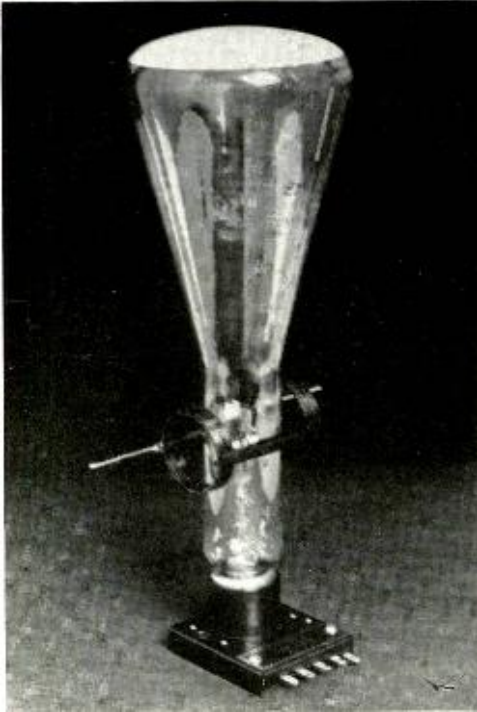
The cathode ray oscillograph tube
