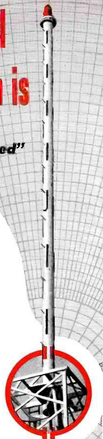
RCA Adjustable Beam High-Gain UHF Pylon—installed
