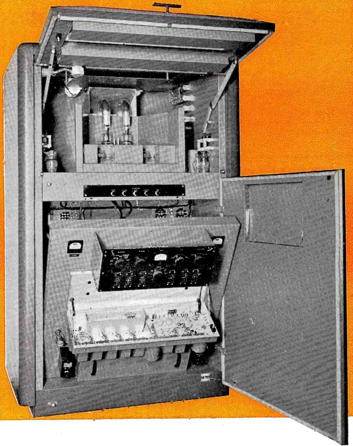
Collins Type 731A 250 watt FM transmitter
