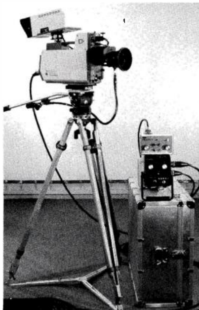
MNC-71CP with 5" viewfinder, mounted on Universal 2030 fluid head tripod (equipped with double handles). Also shown: Remote Production Control Unit and Remote Control Panel ("Paint Box"), camera case and related accessories.
