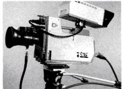
MNC-71CP with 5" viewfinder, mounted on Universal 2030 fluid head tripod (equipped with double handles). Also shown: Remote Production Control Unit and Remote Control Panel ("Paint Box"), camera case and related accessories.
