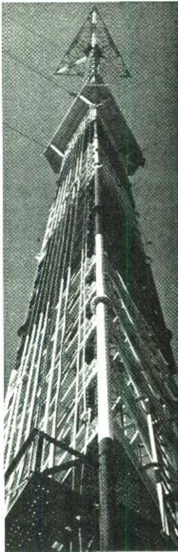
Candelabra ® tower carries 3 antenna as high as 1549' above ground for KCRA-TV, KOVR, KXTV.
