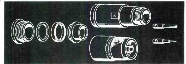
NUT RETAINER TYPE — 75 OHM CONNECTOR
