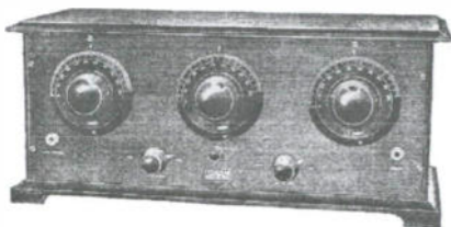
Figure 1. A Freshman Masterpiece, ca. 1924. This 5-tube Tuned Radio Frequency (TRF) set used two TRF stages, a detector and two stages of audio amplification.
