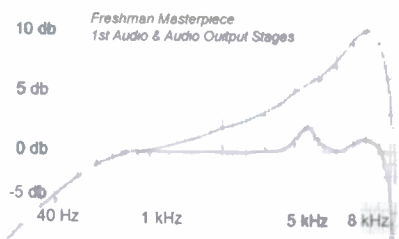
Figure 3. The audio frequency response for the 1st audio and audio output stages.
