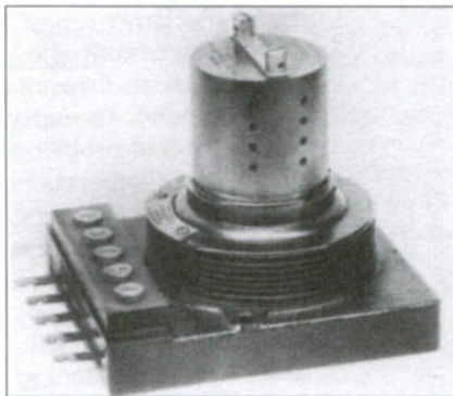
Figure 2. Bell model 3A mechanical repeater.
