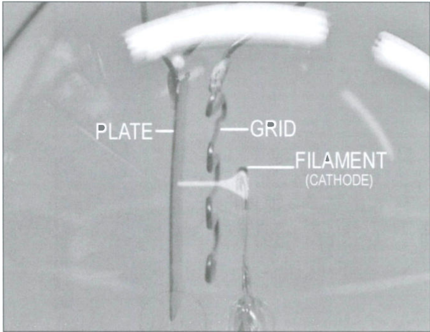
Figure 4. Electron flow within a vacuum tube (see text).
