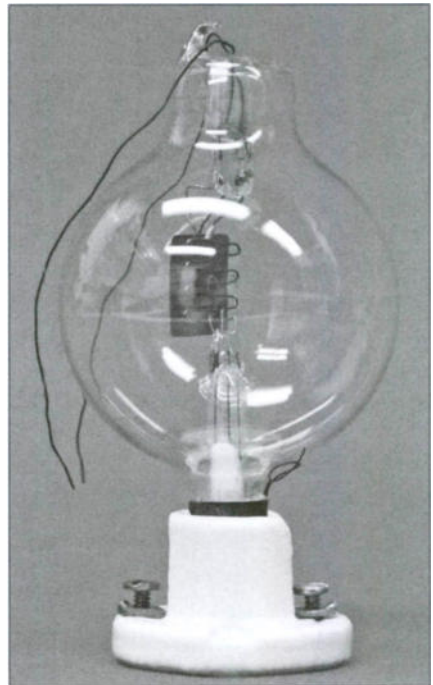
Figure 3. The deForest single-wing Audion tube.
