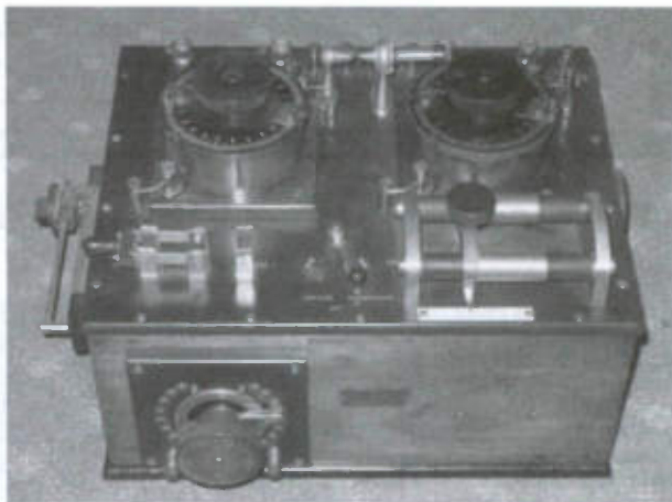
Figure 2. American Marconi 103 receiver.
