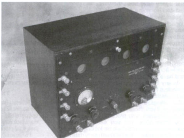
Figure 11. The Marconi 4 VA Four Step Valve Amplifier.
