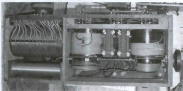
Figure 8. An inside view of the multiple tuner.
