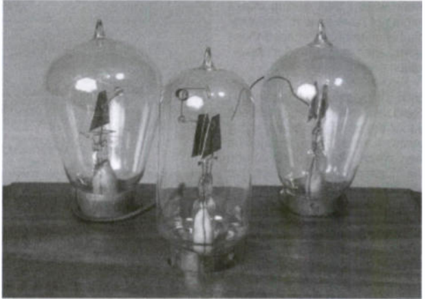
Figure 1. Three different American Marconi Fleming Valves.
