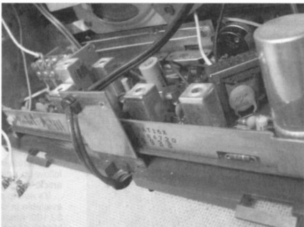
Figure 5. A view of the Zenith Model A411 chassis.
