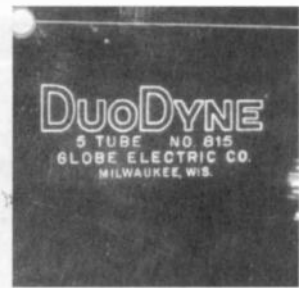
Look at all those knobs... and a meter, too! This Globe Electric DuoDyne 5-tube set sold for $280 in 1924. Without tubes, it sold here for $250. On the right is a close-up of the engraving on the panel.
