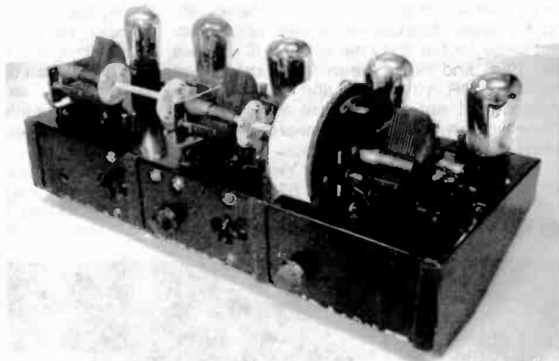
Figure 3. The Model 5-50 chassis. The three ganged variable capacitors can be clearly seen.
