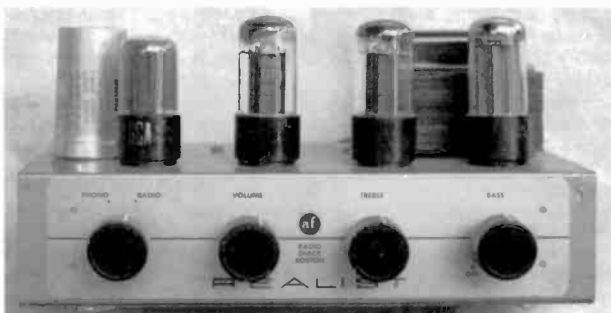
Figure 1. A head-on view of the Radio Shack "Little Jewel" Model LJ-2 amplifier. Note the brand name "Realist" that preceded the better known "Realistic" line.
