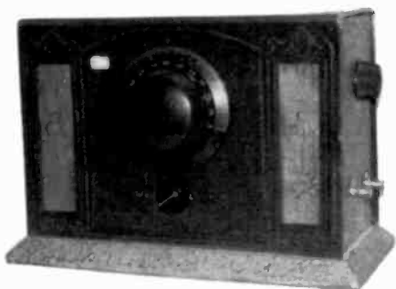
VIKING MODEL 599 – This 5-tube radio was manufactured by the Viking Radio Laboratories of Chicago, Illinois, which was part of Ozarka Radio Manufacturers. In 1926, this set sold for $25 without tubes or speaker. The cabinet is made of embossed leatherette over heavy fiberboard. (Wally Worth – Wollaston, MA)
