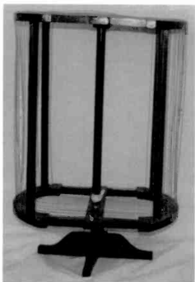
This is a repro of the Radiola AG-814, one of the larger loops that RCA manufactured.
