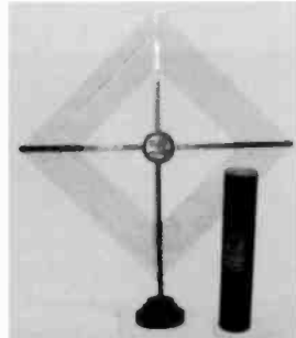
This original 1924 Portena loop folded up and fitted into a cardboard tube that was included.
