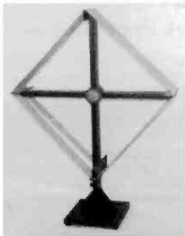
A repro of a Federal Standard Radio Products loop.
