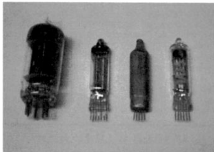
Figure 2. The radio's tubes, from left to right: a miniature 3S4 and three subminiatures — a 1V6, a 1AH4 and a 1AJ5.
