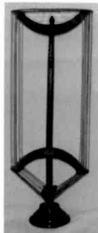
Repros of two of the taller type of loop antennas are shown here. At left is the familiar style that fitted into the top of the 1925 RCA Radiola 25 receiver. At right is the self-standing, bank-wound, Fiat Type "C" made by Radio Appliance Corp.
