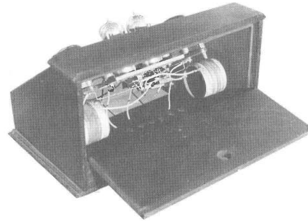
Figure 3. The Nyaccoflex Model R2 with the rear access panel pulled down to expose the two-tube chassis.
