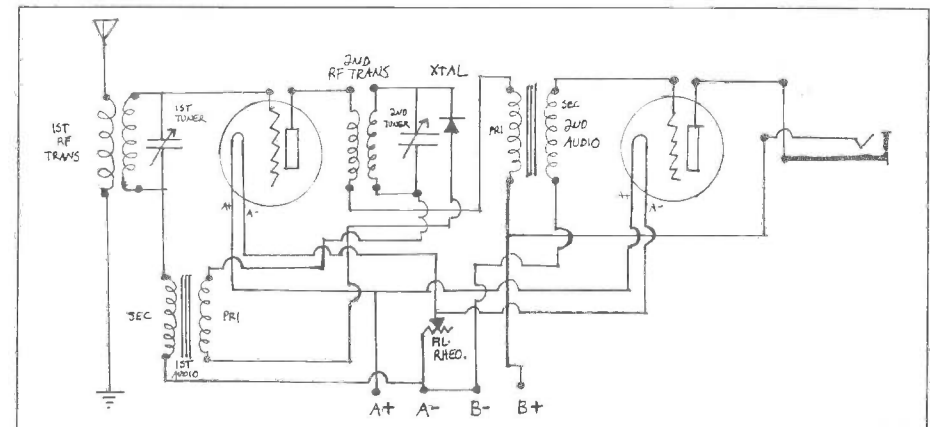
Figure 5. Schematic diagram of the Nyaccoflex Model R2. (Courtesy of Scott MacWilliam).
