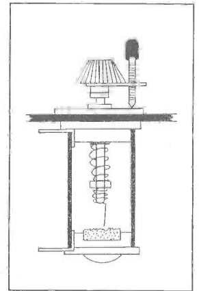
Figure 4. Cross section of the Nyaccoflex crystal detector. (Drawn by Scott MacWilliam).
