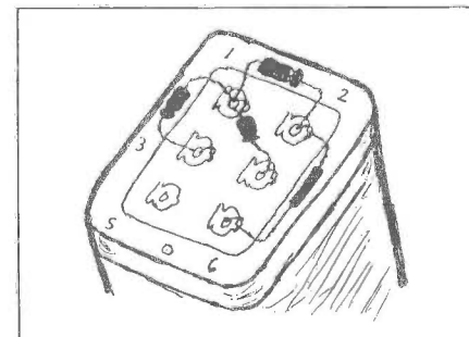
Figure 4. Internal wiring of Philco filter condenser, Part No. 4235, used in Model 20.
