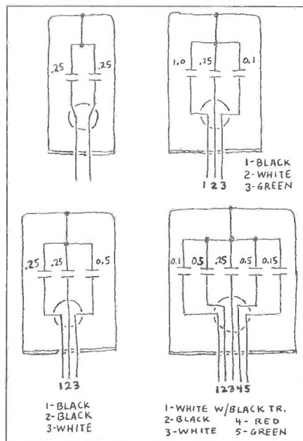
Figure 2. Examples of Philco condenser can hookups. (Top left), Part No. 3557, used in Model 20 and the early Model 112. (Top right), Part No. 03327, used in Model 90 with one Type 47. (Bottom left), Part No. 03029, used in Model 90 with two Type 45s. (Bottom right), Part No. 03915, used in Model 38.
