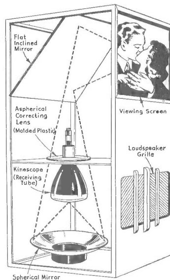
Figure 3. The projection television system for the General Electric Model 901, developed by the RCA Laboratories. ("Television: The Eyes of Tomorrow", 1945.)
