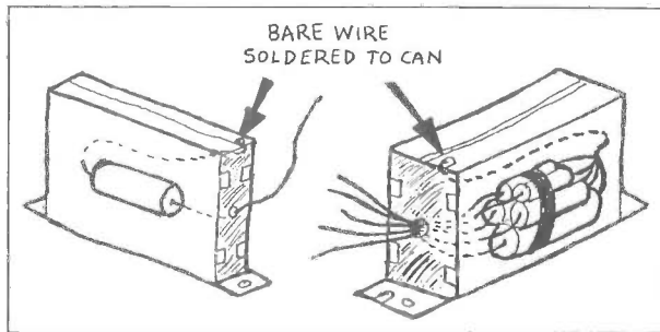
Figure 1. Philco condenser cans. (Left), Part No. 3583, 0.5 mfd, used in Models 20, 70 and 112. (Right), Part No. 06624, 0.05, 0.05, 0.09, 0.09, 0.25 mfd, used in Model 89.
