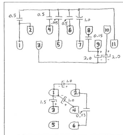
Figure 3. Capacitor replacement layouts for Philco condenser cans. (Top), Part No. 4235, used in Model 20. (Bottom), Part No. 3754, used in Models 111, 112, 211 and 212.
