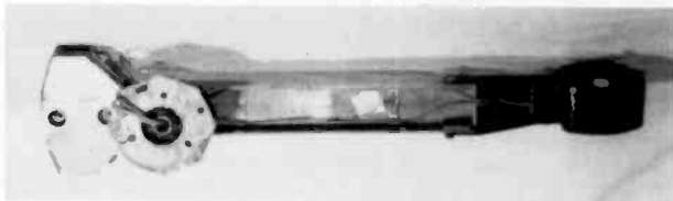
Figure 2. An underside view of the arm, pickup and heavy counterweight of the Western Electric Model 4A phonograph pickup.
