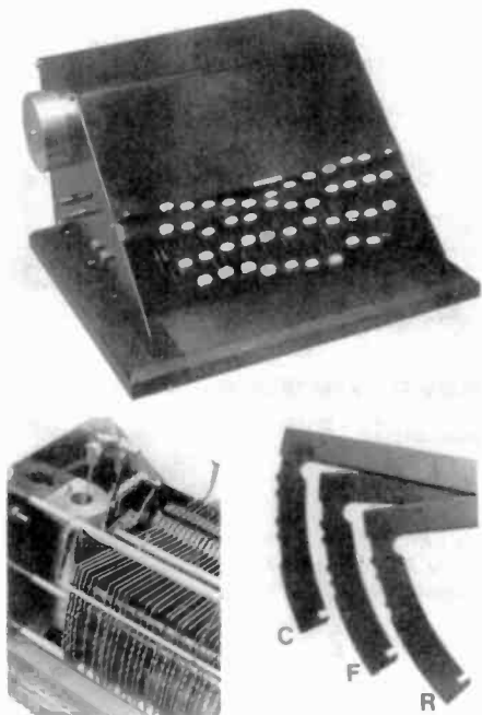
Figure 6. Traeger's ingenious solution for the Morse code illiterate. Not unlike a standard typewriter (top), the keys activated steel arms with a working face cut to required long and short spacings (lower right). The internal view (lower left) shows the oil-filled dash pot necessary to produce smooth movement of the keyed arms.
