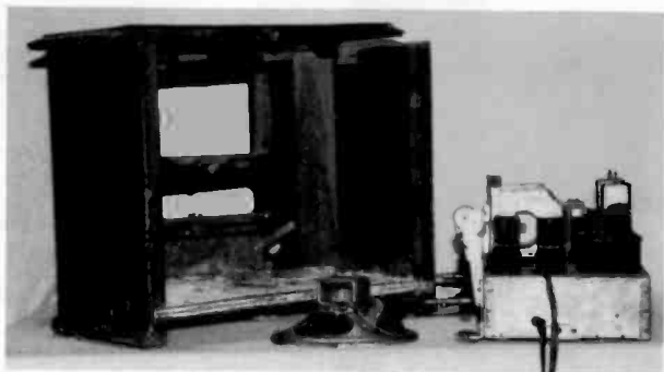
Figure 1. One of the two 1939 RCA Model T-80 radios as found.
