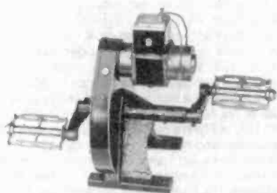
Figure 3. Traeger's solution to the outback's isolation was this prototype of a pedal-operated generator unit for radio sets. Electro-mechanical work was Traeger's specialty.
