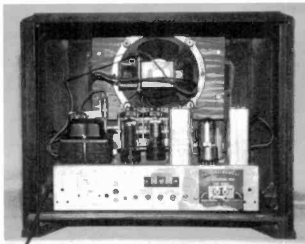
Figure 3. The rear of the completely restored RCA Model T-80.
