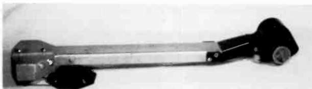
Figure 1. This Western Electric Model 4A transcription-type phonograph pickup head, arm, and counterweight assembly is 17" long.
