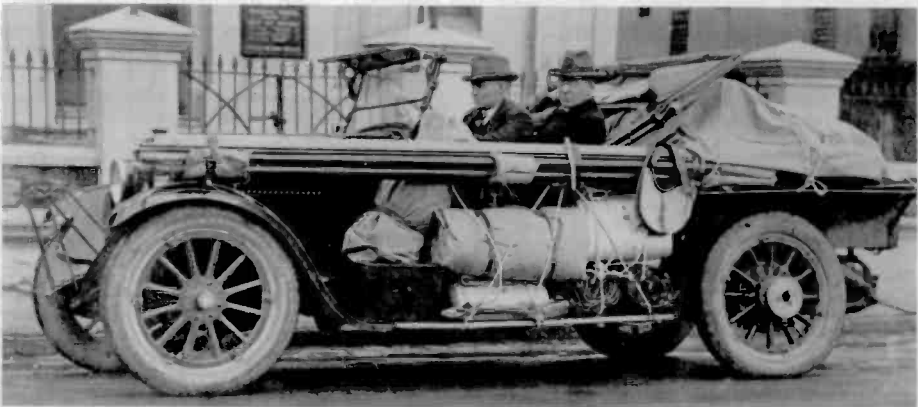
Figure 1. John Flynn (right) and George Towns leave Adelaide in the laden Dodge buckboard, June 1925. Note the pulley built into the rear wheel hub to drive Traeger's generator.
