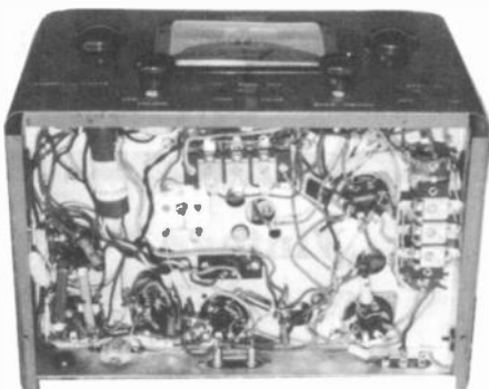
Figure 3. This under-chassis view accents the simplicity of the EC-1. Its uncluttered parts placement makes it a good candidate for the novice restorer.
