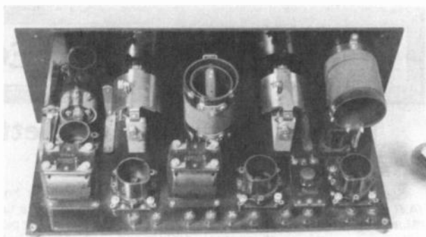
Figure 3. An interior view of the Samson kit. Note that all components are mounted but unwired.
