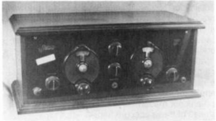
Figure 2. A Samson 4-tube Model T/C kit partially assembled in a home-brew mahogany cabinet.
