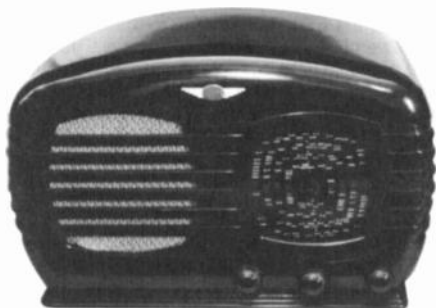
TASMA MODEL 1001 – This 1936 Australian-made Bakelite radio has an AC chassis that requires 240 volts. It uses 4 tubes —Types 6A8, EBF2, EL3, and 5Y3. The set operates on four bands. ( Keith Dennison – Victory Mills, NY )
