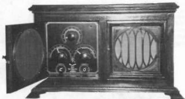
Figure 4. A front view of the radio, including its control panel.
