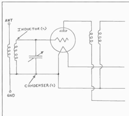
Figure 1. Partial schematic diagram of a radio's front-end connected to a long-wire antenna.
