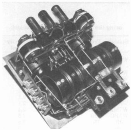
Figure 7. An under-chassis view of the radio.
