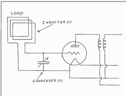
Figure 2. Partial schematic diagram of a radio's front-end connected to a loop antenna.
