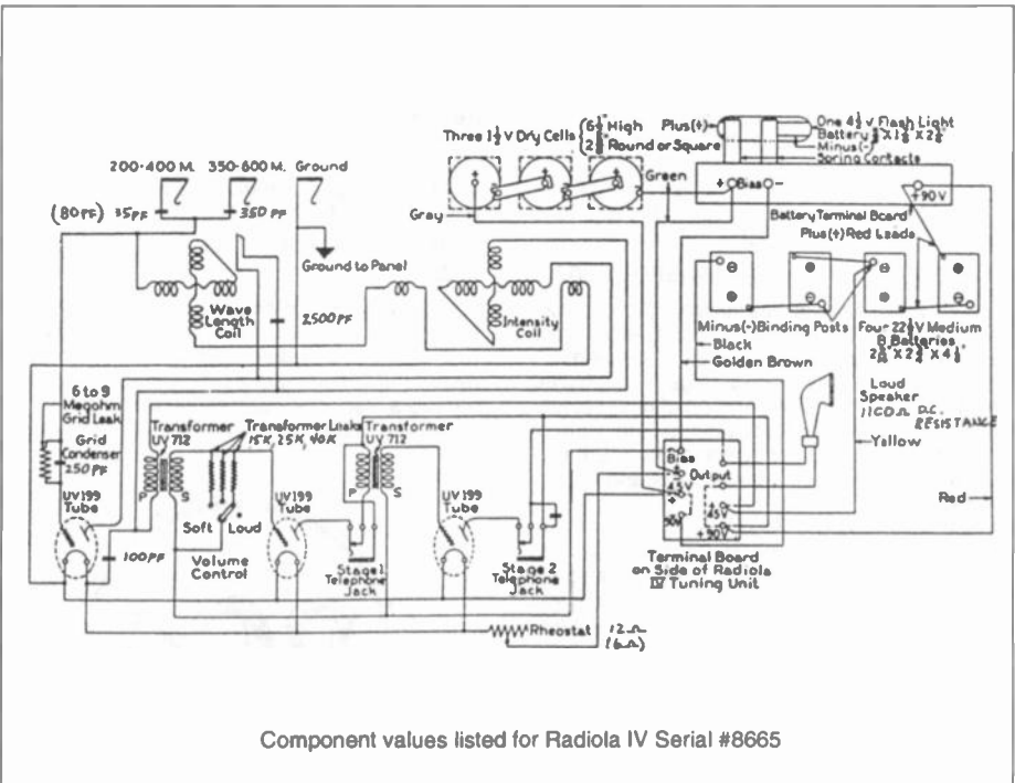
Figure 8. Schematic wiring diagram of the Radiola IV.
