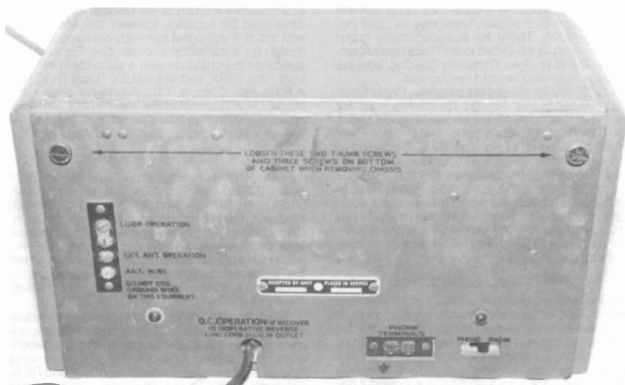
Figure 4. The back of the Crosley REO showing various connections and a Navy acceptance tag.
