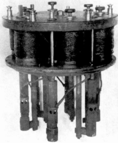
Figure 4. The Arc Fone had 6 series-connected carbon arcs, fired under alcohol and kept trimmed by an electromagnetic lifting system.
