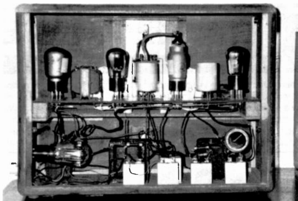
Figure 4. A rear view of the assembled set.
