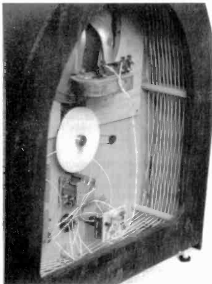
Figure 3. Rear views of the one-tube transistor cathedral radio showing the components used, including the built-in loop antenna.
