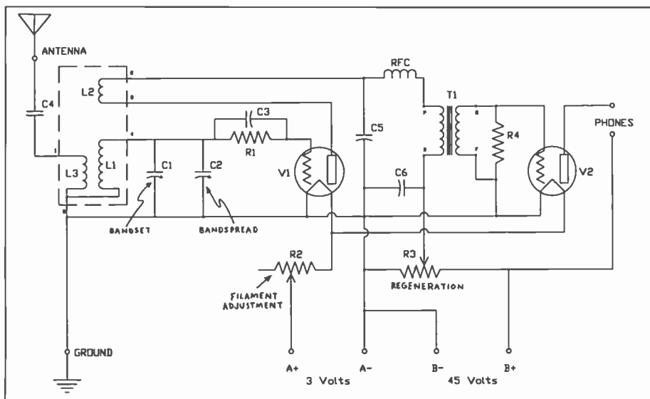
Figure 2. The schematic for the Doerle 2-tube home brew.
