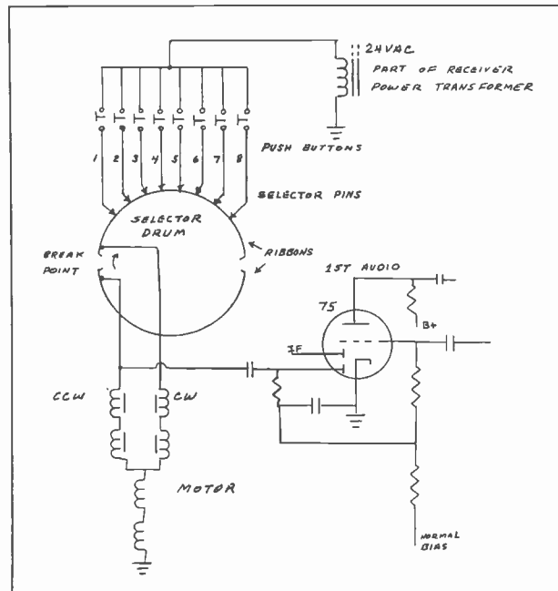
Figure 5. Electro-mechanical schematic of the Truetone Model D-727 tuning system.
