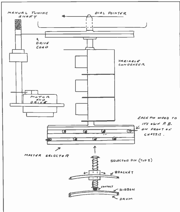
Figure 4. Mechanical diagram of the Truetone D-727 tuning device.
