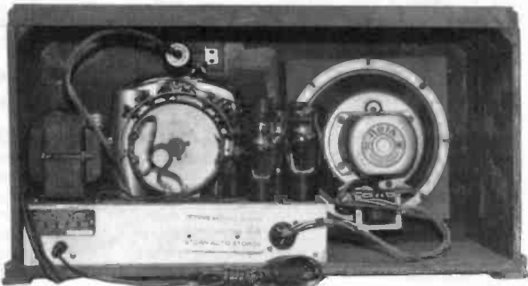
Figure 2. Rear view of the Truetone D-727.
