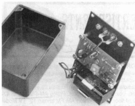
Figure 2. Inside view of the Active Antenna Model AA-10.
