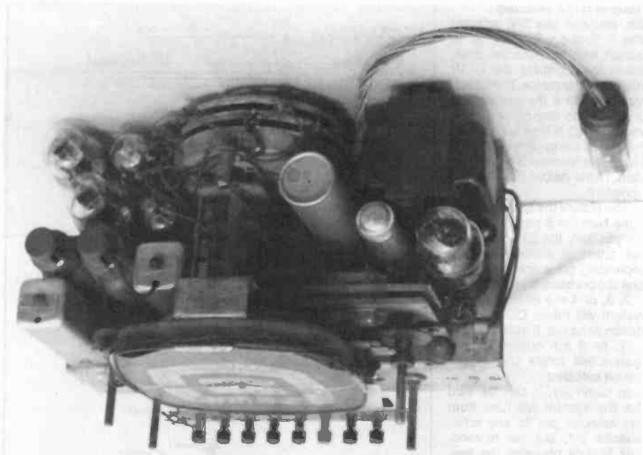
Figure 3. Top view of the Truetone D-727 chassis showing the tuning component lineup behind the dial.
