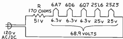
Figure 2. Tube heaters wired in series with a voltage-dropping resistor for 120 volt operation. Note: All tube heaters rated at 0.3 amperes.
