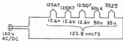
Figure 1. Tube heaters wired in series for 120-volt operation. Note: All tube heaters rated at 0.15 amperes.
