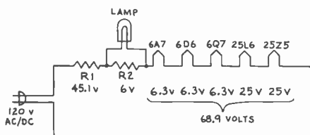
Figure 4. Tube heater circuit for lamp and voltage-dropping resistor. Note: All tube heaters rated at 0.3 amperes. R1 = 150 ohms. R2 = 20 ohms.
