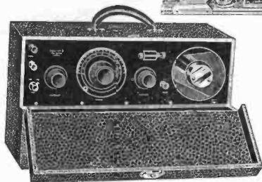
Figure 8. Telmaco Acme P-1 Portable Receiver (reproduced from an insert to a 1923 Telmaco catalog.)
