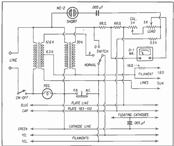
Figure 2. The ASD Model TV-20A Tube Tester circuit diagram.
