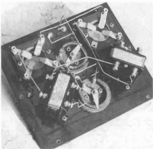
Figure 6. Interior view of the Telmaco Type BA amplifier.
