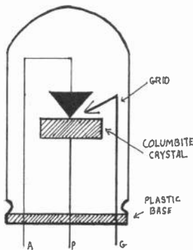
Figure 1. Fips' diagram for the grid crystal tube.
