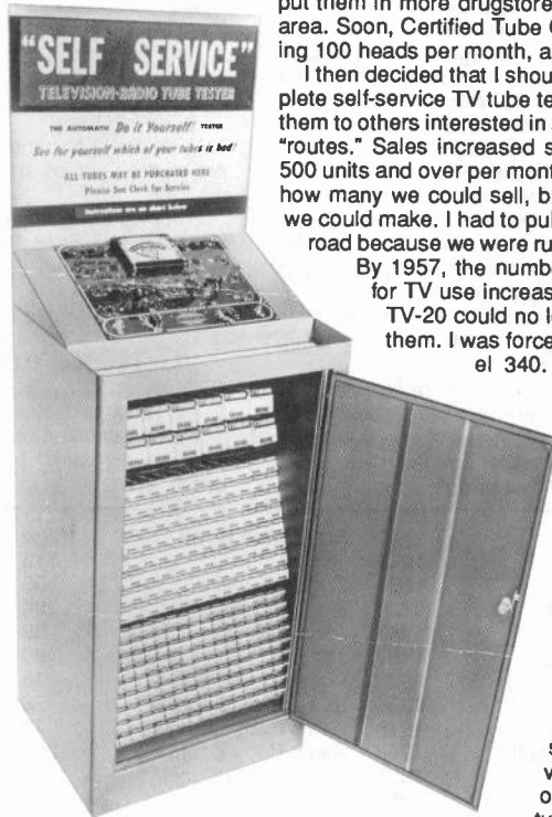
Figure 1. The ASD Model TV-20 Tube Tester.
