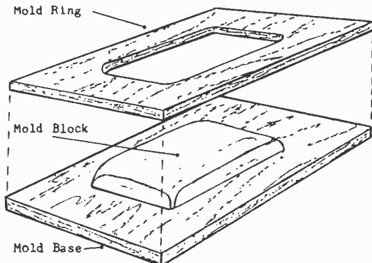
Figure 2. Mold assembly.
