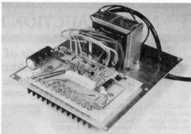
Figure 2. Interior view of the ARBE-III Battery Eliminator showing the rugged, custom-wound power transformer and printed circuit board.
