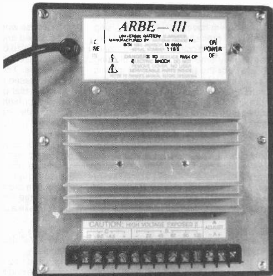
Figure 1. The ARBE-III Battery Eliminator. The sample unit sent to A.R.C. for evaluation used standard panel screws. Purchased models have tamper-proof screws.
