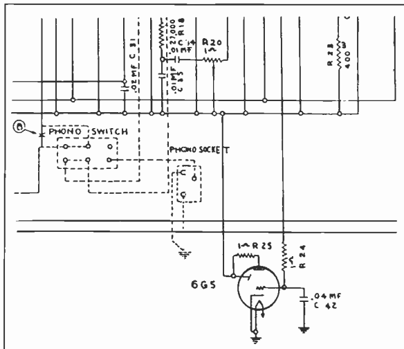
Figure 1. A section from a Stromberg-Carlson schematic, ca. 1937, showing the 6G5 tube area containing the strange code.
