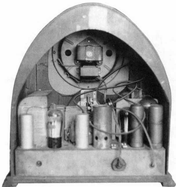
Figure 3. Rear view of the Philco Model 90 cathedral showing the speaker and chassis layout.
