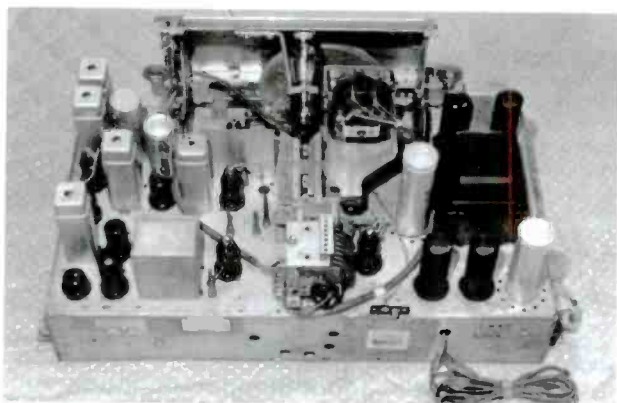
Figure 3. The rear view of the RCA Model 816K chassis shown in Figure 2. The components were left intact, whether repair was needed or not, to retain the original look, even to replacing the color-coded wiring.
