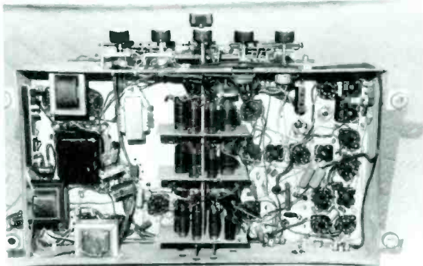
Figure 4. The underside view of the RCA Model 816K chassis. The open audio driver transformer has been replaced with a modern unit that fits inside the old case to retain the original appearance.
