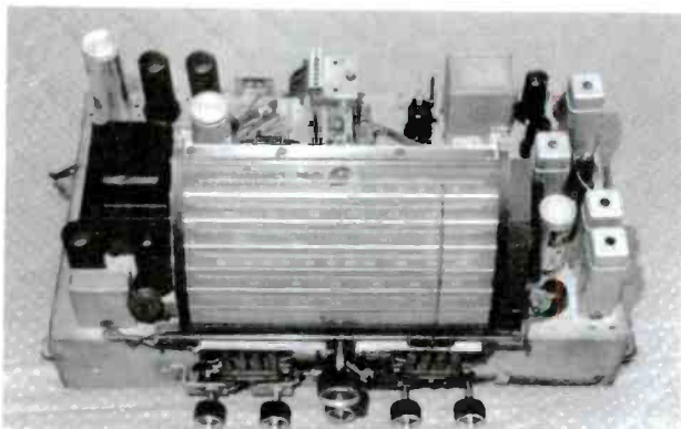
Figure 2. The restored chassis of the "basket case" 816K. Note that the knobs shown are not original, and are shown here for temporary use only.
