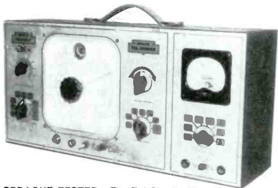
SPRAGUE TESTER - The Tel-Ohmike Model 16 condenser and resistor checker was made by Sprague in 1940. It has an internal power supply for up to 1600 volts and magic eye for null meter indicator. (Walter Worth - Wollaston, MA)
