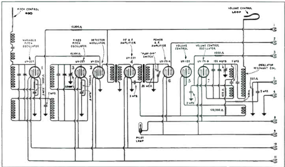
Figure 4. Schematic diagram for the RCA Theremin, Model AR-1264; reprinted from the RCA Victor Service Notes for 1929-1930 (The "Red Book", First Edition, copyright November, 1929; Service Division, RCA Victor Co., Inc., Camden, New Jersey).
