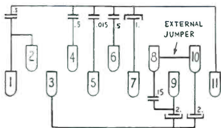
Figure 1. Capacitor replacement layout for Philco condenser cans, part No. 3754.
