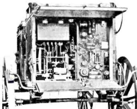
Figure 6. Photograph of the Marconi F-Type wireless telegraphy cart as shown in the 1901 Marconigram reprint.
