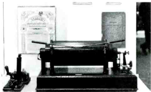
Figure 2. Marconi spark coil, key and antenna switch displayed at the Marconi Co. booth in Washington, D. C. (James Kreuzer Collection)
