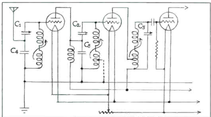
Figure 5. RF stages redrawn from Rider's Vol. 1 to show variometers as variable inductors. C1, C2, C3 are the adjustable fixed-tuning condensers. C4 and C5 are for coupling.
