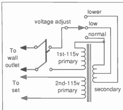
Figure 1. Schematic: Conversion of dual primary transformer to isolation type.
