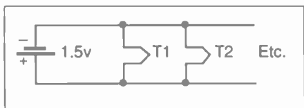
Figure 3. Tube filaments connected in parallel with each other and with a battery.
