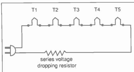
Figure 6. Tube filaments in series with dropping resistor connected with the power line.
