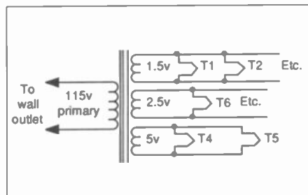
Figure 5. A multi-filament-voltage transformer with tube filaments connected in parallel.
