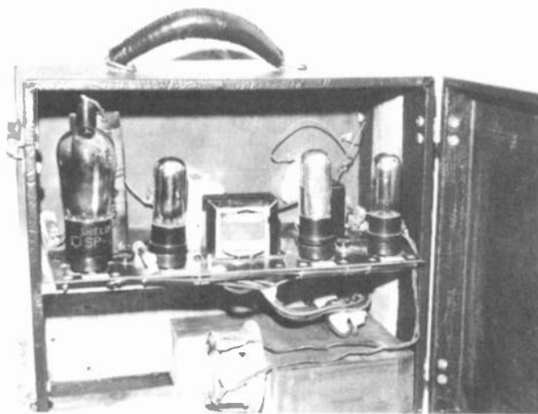
Figure 2. Interior view of 1929 Tom Thumb, showing one 222 SG, three 199's and wooden horn.
