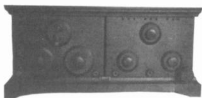
RADIOLA V - Model AR-1300, 175-700 meters. Manufactured by General Electric Corp for RCA. All knobs have GE logo. Lower right has a Murdock honeycomb multiple headphone plug. Note the lid on the top which is often missing from these sets. (Charles Ryan, Mogadore, OH)
