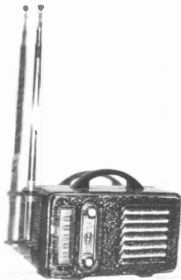
Figure 3. 1947 four-tube Tom Thumb bicycle radio in maroon crackle finish which attached to the handlebars.
