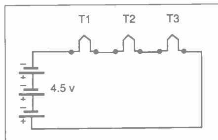
Figure 4. Tube filaments connected in series with each other, and with three batteries in series.
