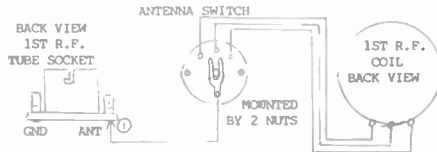
Wiring hook-up for the 3-position antenna switch.
