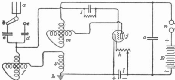
Figure 2. Radiola Senior circuit diagram.
