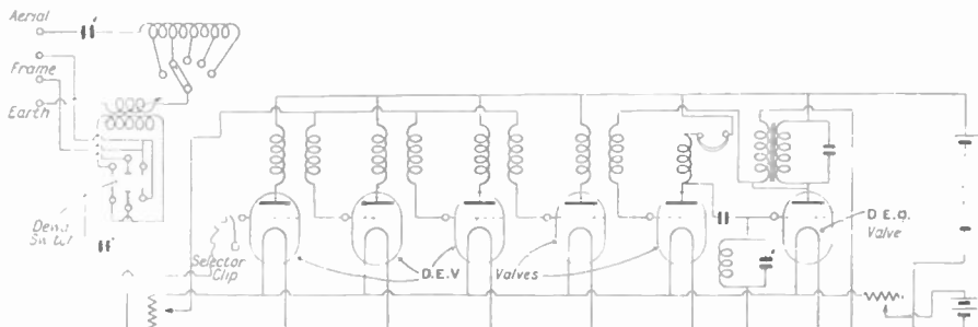
Figure 2. Circuit diagram of the Marconiphone R.B.7 Receiver. The aerial circuit is tuned by means of a series condenser and tapped inductance, and is loose-coupled to a secondary circuit, tuned by a condenser. The loose coupling is partly responsible for the excellent selectivity of the receiver. Regeneration is controlled by a potentiometer (in the lower left of the schematic) which varies the grid voltage. Transformers couple the first four stages of RF amplification in this set. The final stage is coupled by a tuned anode (plate) circuit to the rectifier (detector), the D.E.Q. valve. Note that the audio transformer in the anode of the D.E.Q. valve is coupled back to the grid of the previous D.E.V. valve. This valve serves both as the detector and the audio output (note the headphones in the anode circuit).
