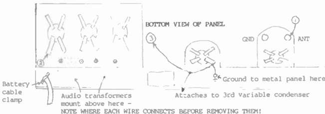
Wiring hook-up for the filament rheostats/on-off switch unit.
