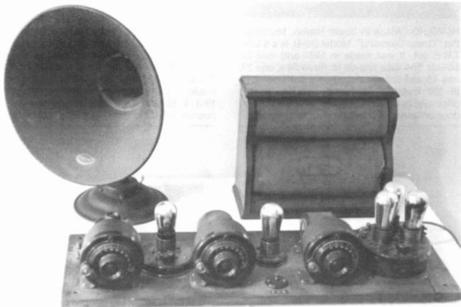
The author used this set-up for DXing. The AK Model "L" horn was frequently disconnected on weak signals in favor of a Dictogrand cylindrical speaker. Photo by Lance Funderburk.
